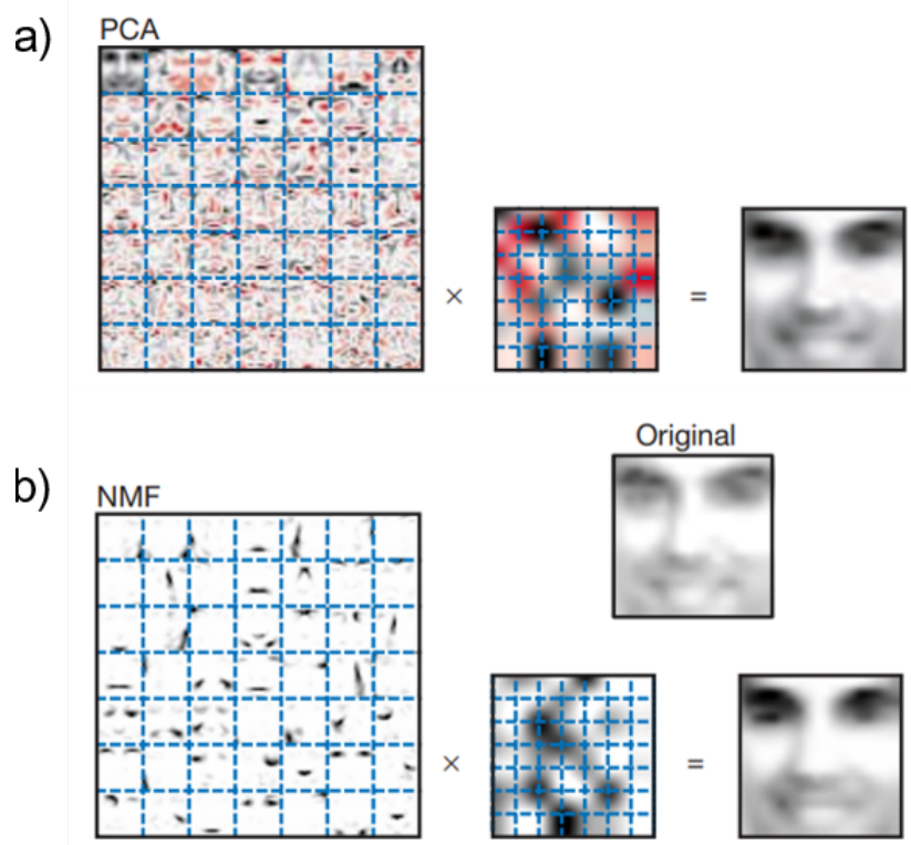
Figure 5.12: NMF learns resembling part objects of faces, whereas principal components analysis (PCA) learn holistic representations. Positive values are illustrated with black pixels and negative values with red pixels. The coefficients of the linear superposition (scores) are shown next to each montage
