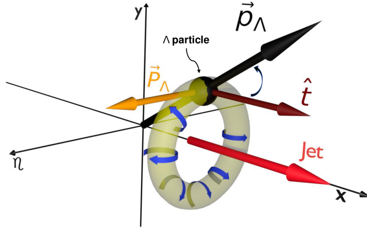
Figure 3.5: Illustration of the vectors involved in the analysis of the \mathcal{R} observable. The dot product between the vector \vec{P}_\Lambda and (\hat{t} \times \vec{p}_\Lambda) will maximize the polarization values in the direction of the vorticity ring, making \overline{\mathcal{R}}_\Lambda^t a suited observable to describe the polarization effects in the transverse plane of the jet.
