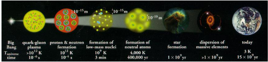
Figure 2.2: History of the universe [32]. We note that the Quark-Gluon Plasma is the first matter formed after 10^{-6} s of the big bang, followed by the formation of protons, neutrons and low mass nuclei.
