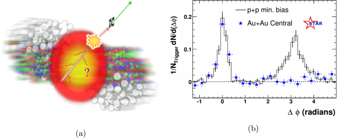
Figure 1.1: (a) Schematic representation of a jet quenching inside the Quark-Gluon Plasma. Due to hard interactions, a back-to-back jet is formed near the QGP. One component goes through the relativistic fluid, being suppressed, while the other proceeds unquenched [21]. (b) Comparison of azimuthal distribution for pp and Au–Au collision. The left peak, representing the near-side jet, is similar in both systems. The right peak, representing the away-side jet, is suppressed in the system formed in Au–Au collisions, whereas no suppression is observed in pp collisions where no QGP formation was expected. Adapted from [20].
