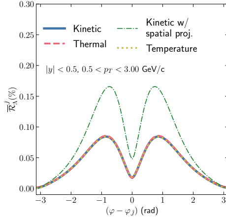
Figure 5: \vec{\mathcal{R}}_\Lambda^j (see Eq. 9) computed from \Lambda -polarization calculations using four types of vorticity tensor.
