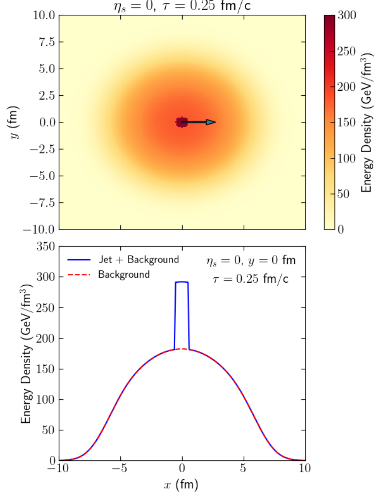
Figure 4.3: Initial condition of the thermalization on top of the background fluid. The top plot shows the energy density as a function of the positions x and y , for \eta_s = 0 . We note the jet thermalization as the high-density region centered at (x, y, \eta_s) = (0, 0, 0) . The bottom plot shows the projection of the initial energy density (red curve) with the jet thermalization (blue curve), for y = 0 fm and \eta_s = 0 .
