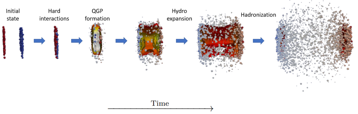
Figure 2.1: Stages of a heavy-ion collision. The initially Lorentz contracted nuclei accelerate at each other, yielding a hard collision and forming the Quark-Gluon Plasma. The medium then expands according to relativistic hydrodynamics up to a point where the quarks and gluons have enough energy to combine into hadrons and free-stream from the system [29].
