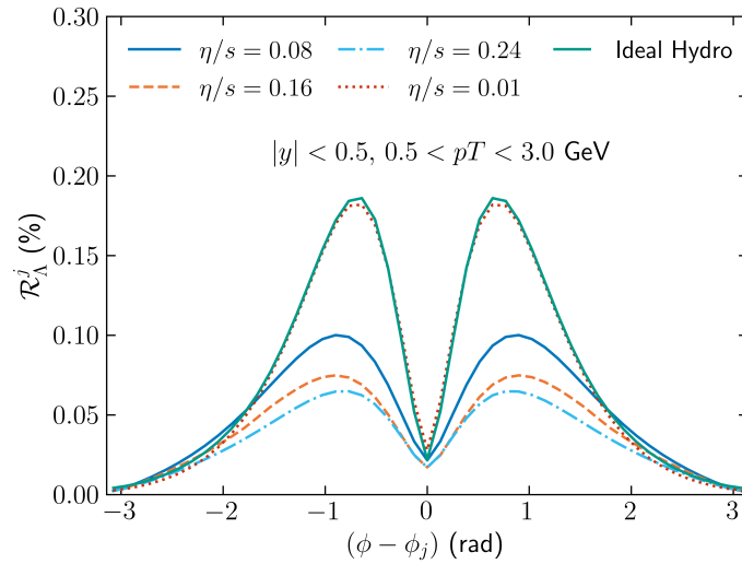
Figure 5.13: \overline{\mathcal{R}}_{\Lambda}^{\hat{t}} parameter comparison for different values of shear viscosity. The y axis represents the percentage of the observable \overline{\mathcal{R}}_{\Lambda}^{\hat{t}} and the x axis the azimuthal angle relative to the jet direction. We see that the increase in the viscosity also interferes in the values of \overline{\mathcal{R}}_{\Lambda}^{\hat{t}} , and consequently, in the polarization of \Lambda .
