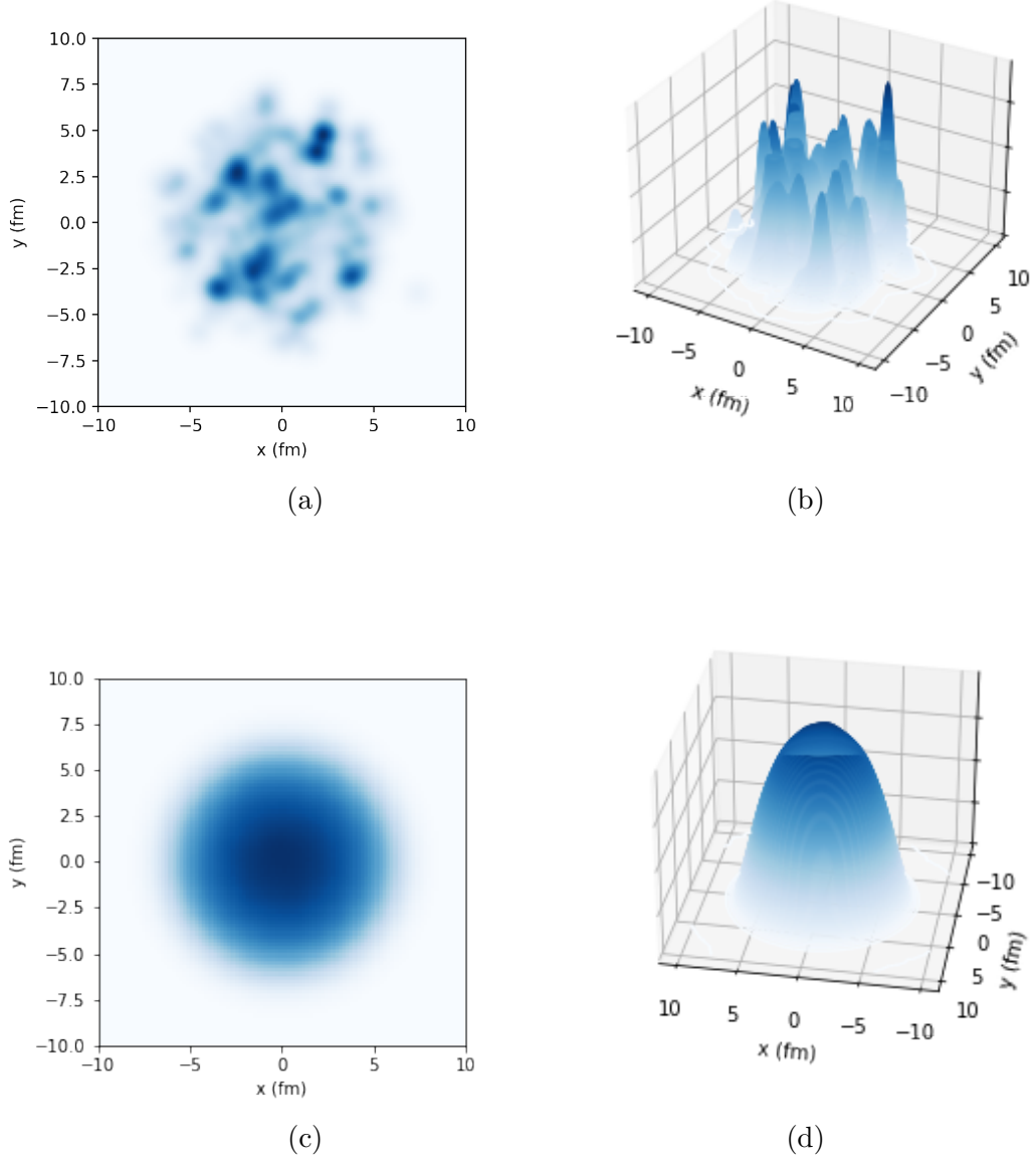
Figure 4.1: Energy density profiles from T RENT o simulations for two scenarios of initial conditions. (a) shows the energy distribution for a single event as a function of x and y , projected for \eta_s = 0 , and (b) its surface view. We note the formation of non-uniform structures. (c) and (d) shows a similar scenario, but for a smooth initial condition, averaged over a thousand events.
