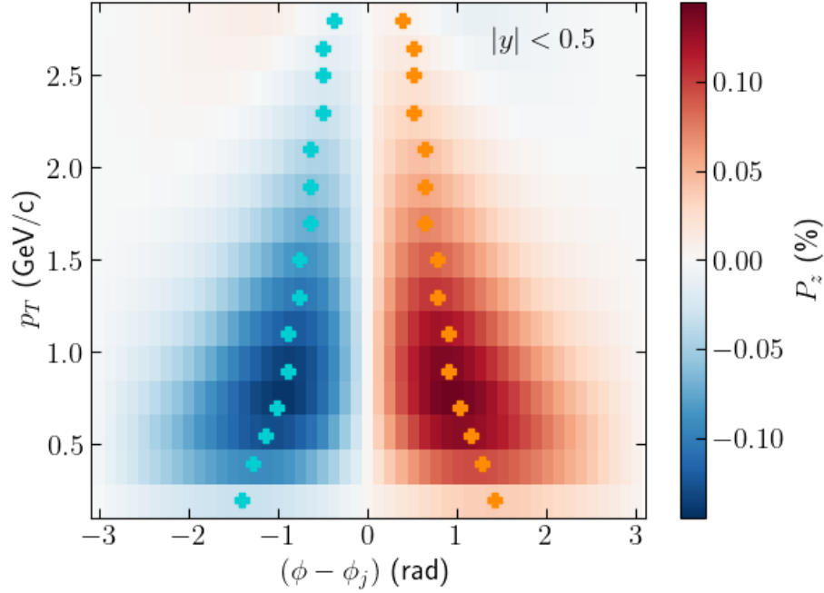
Figure 5.11: Distribution of the weighted average of the component P_z of the Lambda polarization, as a function of the momentum p_T and the azimuthal angle relative to the jet direction. The colored dots represent the bins of p_T where |P_z| has a maximum value.
