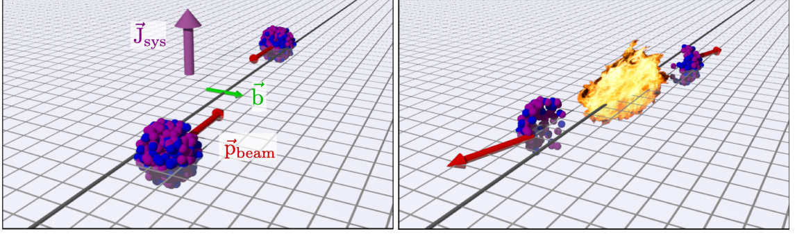
Figure 3.1: Sketch of a collision and the formation of the fireball with total angular momentum represented by \hat{J}_{sys} . The left Fig. represents the two nuclei before the collision, with impact parameter \vec{b} , momentum of the beam \vec{p}_{beam} and momentum of the collision \hat{J}_{sys} = \vec{b} \times \vec{p}_{beam} . The right Fig. shows the formation of the fireball. In a non-central collision, this fireball will develop an angular momentum, and consequently, vorticity in the direction of the total angular momentum \hat{J}_{sys} [25].
