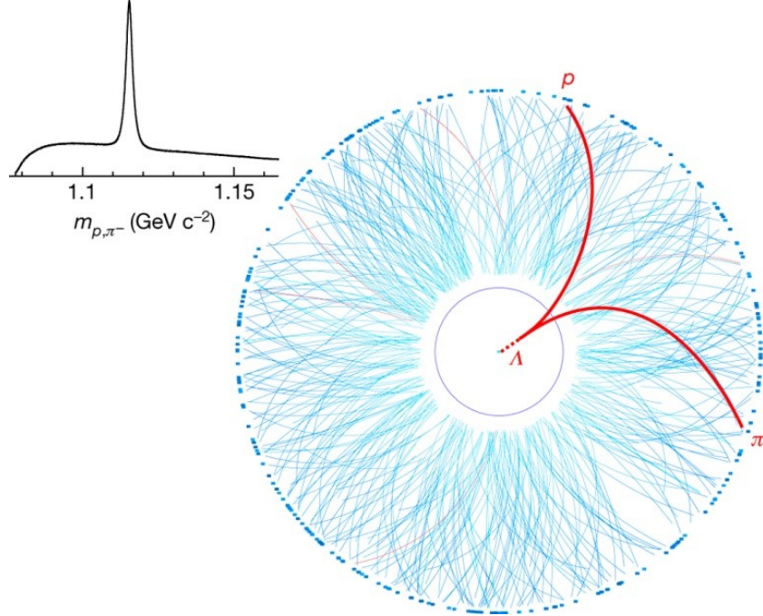
Figure 3.2: Star TPC reconstruction of a Au–Au collision. Particles reconstructed tracks are shown as the curved colored lines. The weak decay of \Lambda into p and \pi is shown in red. The paths are reconstructed based on charged particles's time of flight and ionization left on the TPC. The invariant mass distribution is also shown, indicating a peak at the \Lambda mass, that is, around 1115 MeV [3] .
