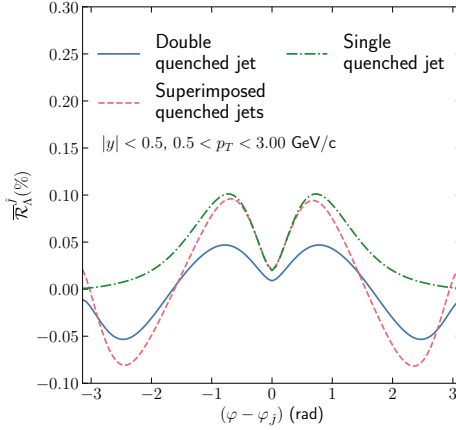
Figure 7: Comparison between the \overline{\mathcal{R}}_\Lambda^j in a double-quenched jet scenario versus the single-quenched jet case. The blue curve shows the result from the simulation and the red one by superimposing two single-quenched jets (shown in green).
