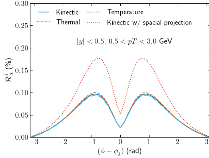
Figure 5.12: \overline{\mathcal{R}}_{\Lambda}^{\hat{t}} parameter comparison for different types of vorticity. The y axis represents the percentage of the observable \overline{\mathcal{R}}_{\Lambda}^{\hat{t}} and the x axis the azimuthal angle relative to the jet direction. The similar values of \overline{\mathcal{R}}_{\Lambda}^{\hat{t}} for the thermal, kinetic, and temperature vorticities indicate that the vorticity is formed, mainly, by gradients of velocity.
