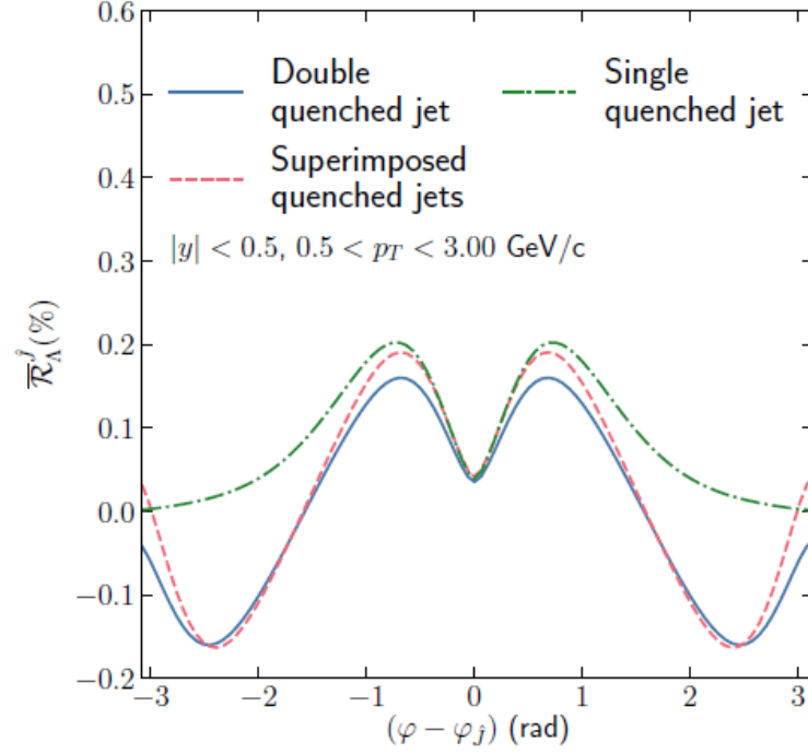
Figure 5.14: \overline{\mathcal{R}}_{\Lambda}^i parameter comparison for different jet thermalization scenarios as a function of the azimuthal angle relative to the jet direction. The green curve shows the case where there's only one jet travelling in the +x direction. The red curve describes the behavior of two superimposed jets, moving at opposite directions. The blue curve shows the scenario where two jets are separated by a distance \Delta x = 1.2 fm in the x axis, also moving in opposite directions.
