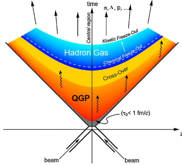
Figure 2.5: Space-time evolution of an ultra-relativistic heavy-ion collision. As the two beams collide, the matter formed goes through the pre-equilibrium phase, the QGP evolution, hadron gas and finally kinetic freeze-out, where the particle free-stream from the system. The yellow area represents the cross-over region, dividing the QGP from the hadronic matter. Adapted from [42].
