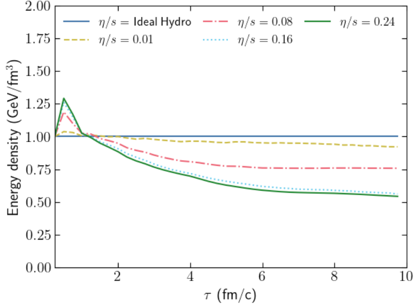
Figure 5.5: Comparison of the maximum value of energy density of the jet as a function of the time \tau , for different viscosity values. All curves have been scaled by the results obtained from the ideal hydrodynamics case. We note that the energy density drops faster for higher values of viscosity.
