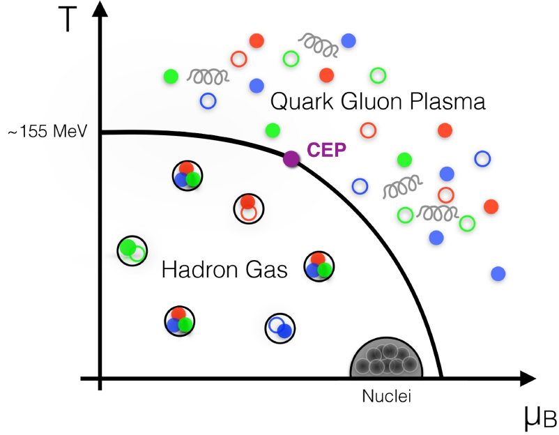
Figure 2.3: Phase diagram of the QCD matter in terms of the temperature T and the baryon potential \mu_B . The Quark-Gluon Plasma phase is separated from the hadronic matter by a phase transition. LHC and RHIC top energies, for example, explore the vanishing baryon potential, while lower energies reaches \mu_B > 0 regions. The critical end point (CEP) represents a second order transition point that possibly marks the separation between the two different states. The location of the CEP is still an open question. Adapted from [38].
