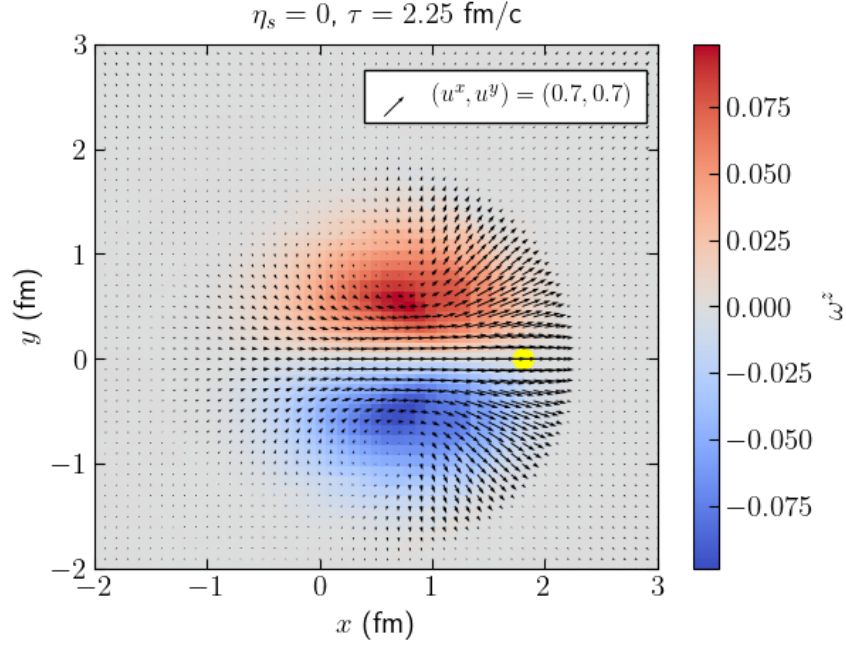
Figure 5.7: Component \omega^z of the vorticity as a function of the positions x and y , for a slice in \eta_s = 0 and time \tau = 2.25 fm/c. The arrows are formed by the components x and y of the four-velocity, with an accentuated curl close to the region of maximum vorticity. The yellow dot represents the position of the thermalized jet in the simulation.
