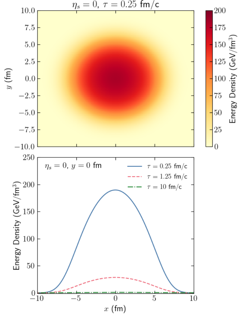
Figure 4.2: Initial condition of the energy density without the jet thermalization. The top plot shows the energy density as a function of the positions x and y , for \eta_s = 0 . The bottom plot shows the energy density profile as a function of x , for y = 0 \text{ fm} and \eta_s = 0 , for three different times of evolution, \tau = 0.25 \text{ fm}/c , \tau = 1.25 \text{ fm}/c and \tau = 10 \text{ fm}/c . We note that the energy decreases as the proper time evolves.
