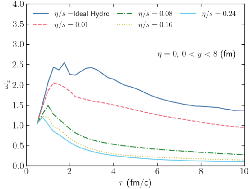
Figure 5.9: Maximum value of the positive part of the component \omega_z as a function of the proper time \tau , sliced at \eta_s = 0 and 0 < y < 8 fm. We note that the vorticity induced by the jet is lower for cases where the medium shear viscosity is higher, but the shape of the reduction curve in time seems to be the same.
