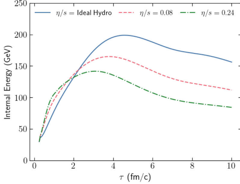
Figure 5.3: Internal energy of the thermalized jet integrated over x , y and \eta_s as a function of \tau . We observe the differences in the energy drop for different values of viscosity. The increase of internal energy is caused by the high pressure gradients the medium imposes to the thermalized jet.
