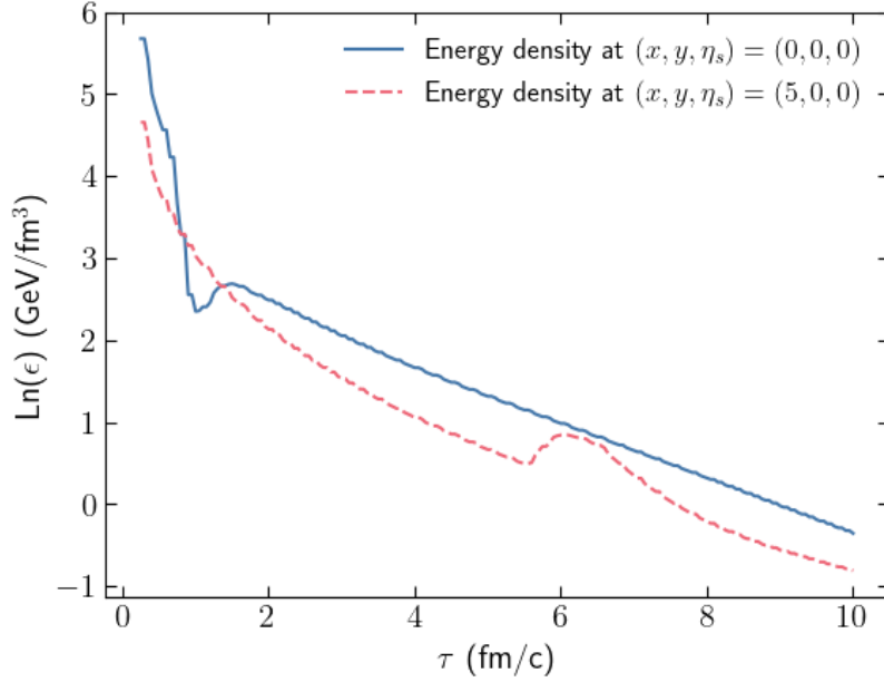
Figure 5.2: Comparison of the natural log of the energy density as a function of \tau for two points of the grid, (x, y, \eta_s) = (0, 0, 0) and (x, y, \eta_s) = (5, 0, 0) . We note that the jet thermalization passes through (5, 0, 0) around \tau = 6 fm/c, represented by the bump in the red curve, and introduces a vacuum region at (0, 0, 0) , represented by the fast drop of the blue curve at the beginning of the evolution.
