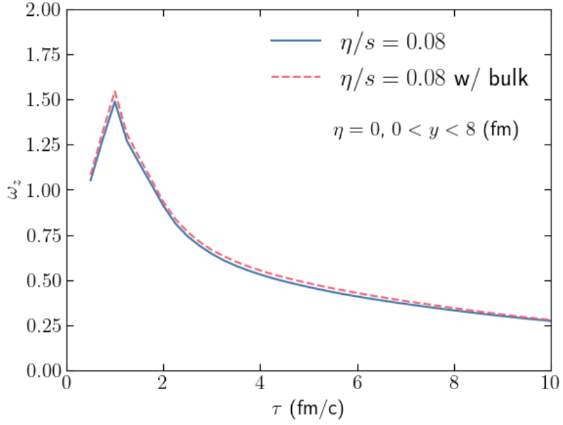
Figure 5.8: Component z of the thermal vorticity versus the time \tau for two different simulations: one considering the shear plus bulk viscosities (red curve), and one considering only the shear viscosity (blue curve). We note that the bulk viscosity has a slight change in the behavior of \omega_z .
