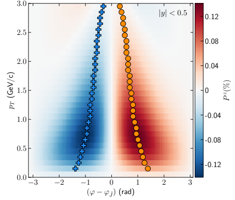
Figure 4: Distribution of the weighted average of the z -component of the polarization ( P^z ), using \Lambda -multiplicity as weight and as function of p_T and the angular distance in the transverse plane. The average considers only data in the range |y| < 0.5 . The orange/blue dots marks the bins where |P^z| is highest for that p_T bin.
