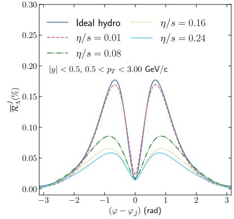
Figure 6: Distribution of \vec{\mathcal{R}}_\Lambda^j (see Eq. 9) for different specific shear viscosities.
