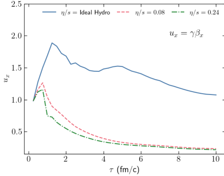
Figure 5.4: Velocity of the jet thermalization as a function of \tau . We note that the velocity is dissipated faster for higher viscosities, while the initial increase of u_x reflects the fast expansion and high pressure gradients the thermalized jet imposes to the medium.
