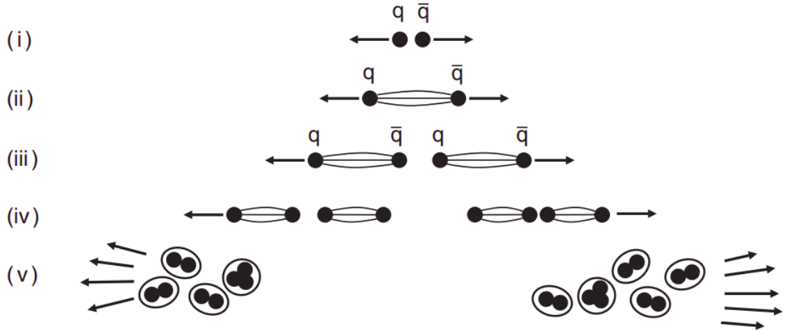
Figure 1.2: Qualitative description of the hadronization process and formation of jet of particles [22]. Steps (i) and (ii) depicts the q and \bar{q} travelling back-to-back and forming the color tube. In steps (iii) and (iv) we show the formation of new quark and antiquark pair from the existing color field, and the subsequent cascade effect forming more q\bar{q} pairs. Finally, in step (v) we have quarks combining into hadrons.
