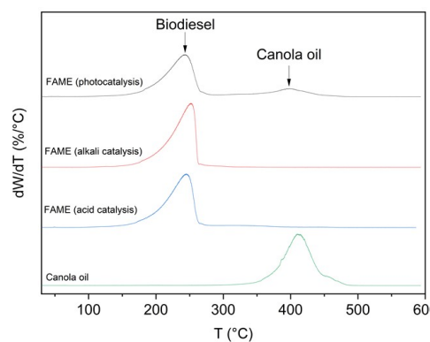
Figure S5. 14. DTA of canola oil and FAME obtained by transesterification catalysed by acid (99% purity), alkali (91% purity), and \text{TiO}_2 irradiated with UVA (73% of purity).
