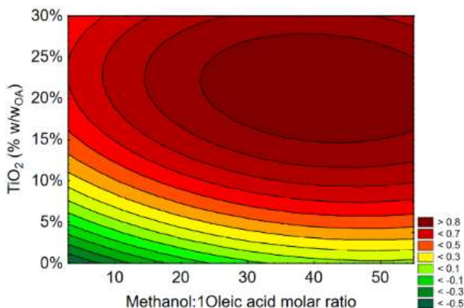
Figure 4. 9. Central composite rotational (CCR) experimental design of oleic acid conversion (%) with methanol to FAME using TiO 2 and UVA irradiation: Surface response contour plots of oleic acid conversion (%) for catalyst content-oleic acid:methanol molar ratio. Temperature: 55°C, TiO 2 content range between 1% and 30% (w/w OA ) and OA:MeOH molar ratio range between: 1:3 and 1:55. Experimental standard deviation ( \sigma ) of \pm 0.00786 .
