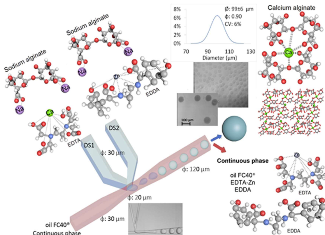
Figure 3. 6. Schematic diagram for the microfluidic droplet synthesis of alginate microbeads, \text{Free}_{\text{catalyst}} , obtained by internal Ion exchange crosslinking. Methylene blue was used to highlight the microbeads. Chemical structures were developed by: Chemdoodle®, and the design was developed by: Sketchup Pro 2021® and PhotoPad Professional v. 6.59®.
