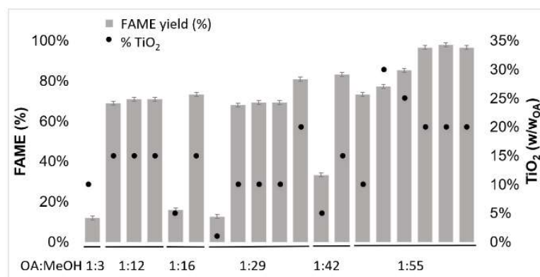
Figure 4. 8. Central composite rotational (CCR) experimental design of oleic acid conversion (%) with methanol to FAME using TiO 2 and UVA irradiation: Oleic acid conversion (%) at equilibrium. Temperature: 55°C, TiO 2 content range between 1% and 30% (w/w OA ) and OA:MeOH molar ratio range between: 1:3 and 1:55. Experimental standard deviation ( \sigma ) of \pm 0.00786 .
