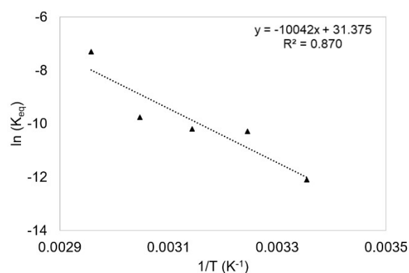
Figure 5. 13. Equilibrium constant for canola oil and methanol transesterification catalysed by \text{TiO}_2 irradiated by UVA. (1TGA mol:55MeOH mol, 20% \text{TiO}_2 (w/w TGL , mathematical model: F2B4).
