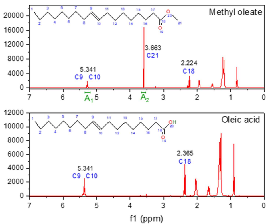
Figure S4. 6. ^1\text{H} -NMR of methyl oleate and oleic acid, respectively. The molecular structures were obtained by ACD/ChemSketch® (Advanced Chemistry Development Inc.).
