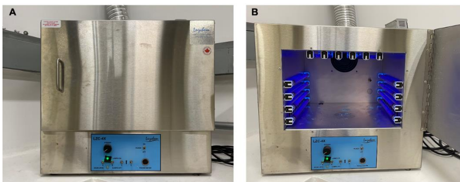
Figure 8. Commercial LuzChem LZC-4X UV Light reactor with 14 UV-light.
