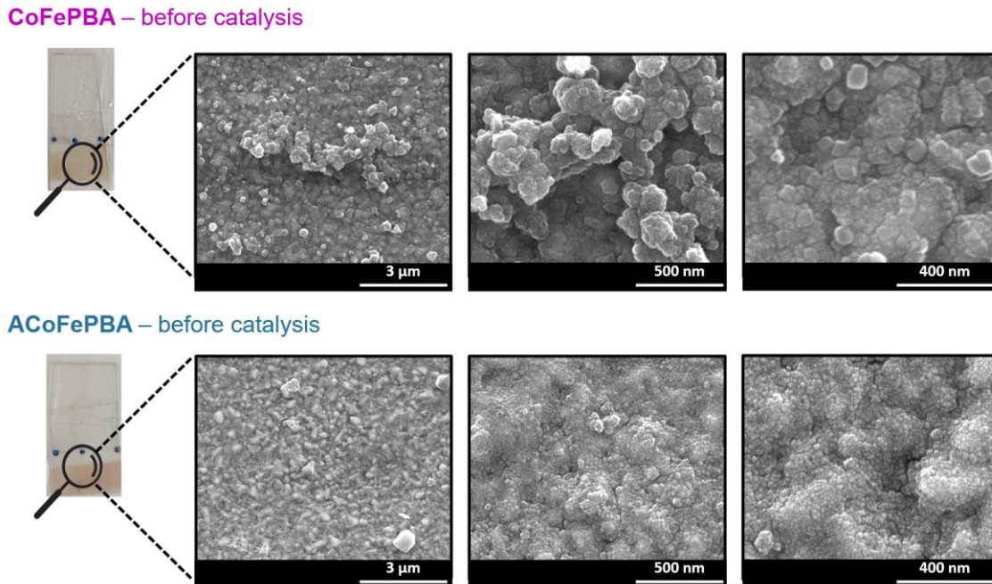
Figure 43. Scanning Electron Microscopy (SEM) of the as prepared catalysts (before catalysis).
