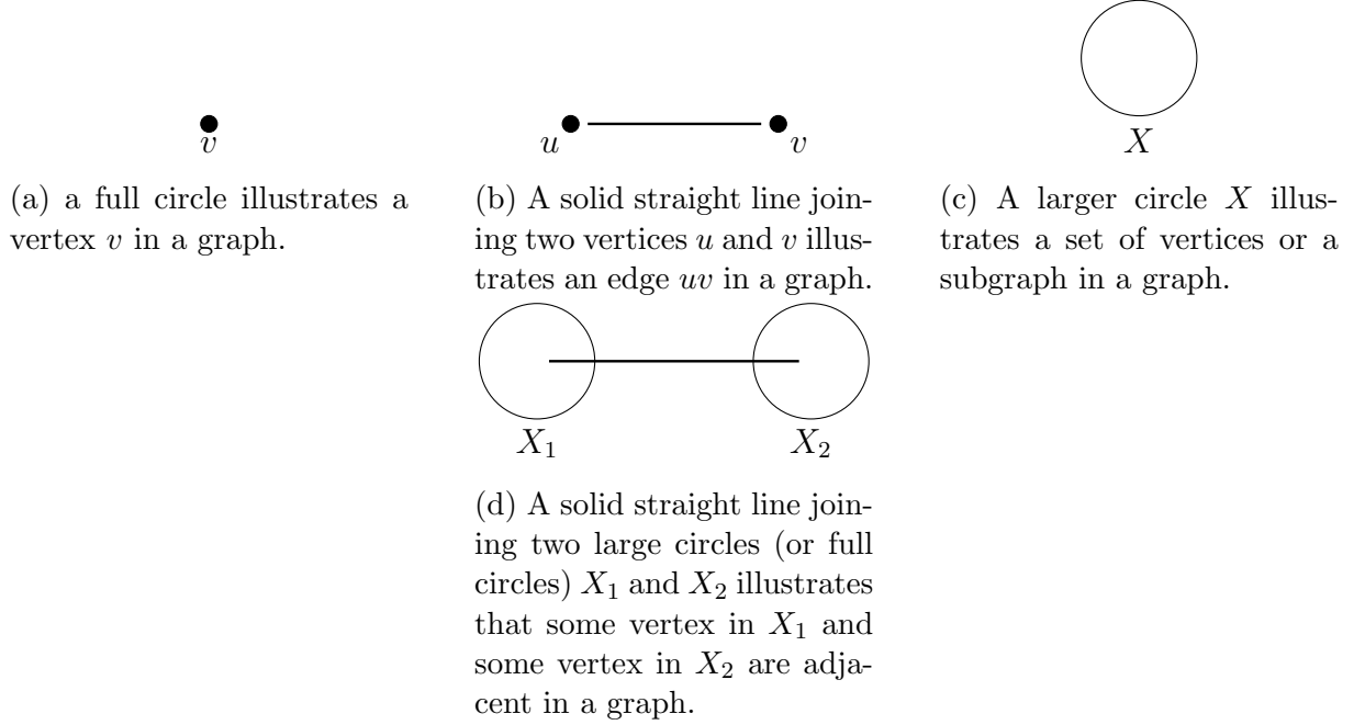
Figure 2.1: Notation used to describe the structure of a graph.
