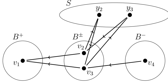
Figure 5.5: Illustration for the proof of Lemma 5.10.
