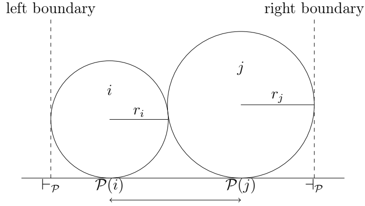
Figure 2.2: Illustration of some basic notations.
