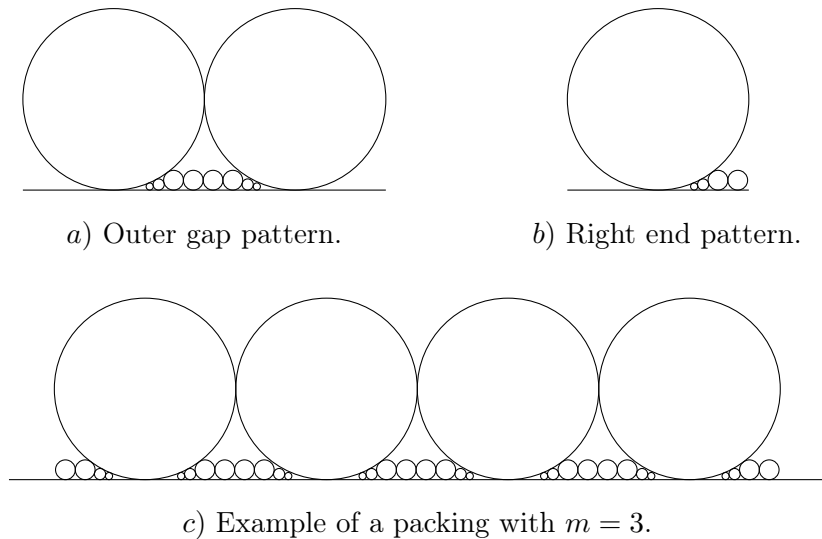
Figure 3.1: Illustration of the unique pattern of a packing with span 2(m+1) .
