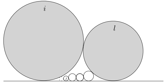
(b) case when there are two or more circles between i and l .
