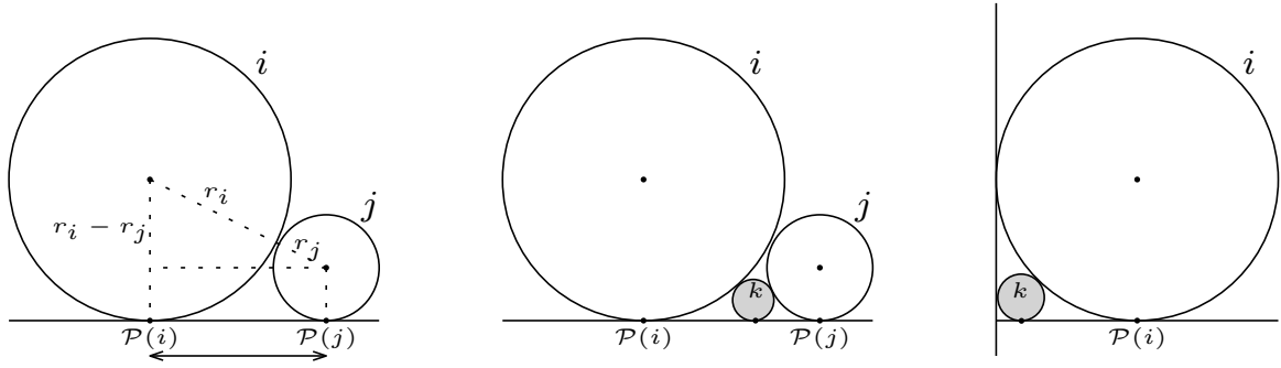
Figure 2.3: Illustration for Lemmas 2.1, 2.2 and 2.3, respectively from left to right.
