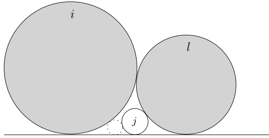
(a) case when j is the only circle between i and l .
