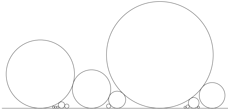
Figure 1.1: Illustration of an in-line packing of Circles.
