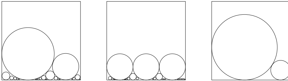
Figure 2.1: Illustration of the In-line Circle Bin Packing problem.
