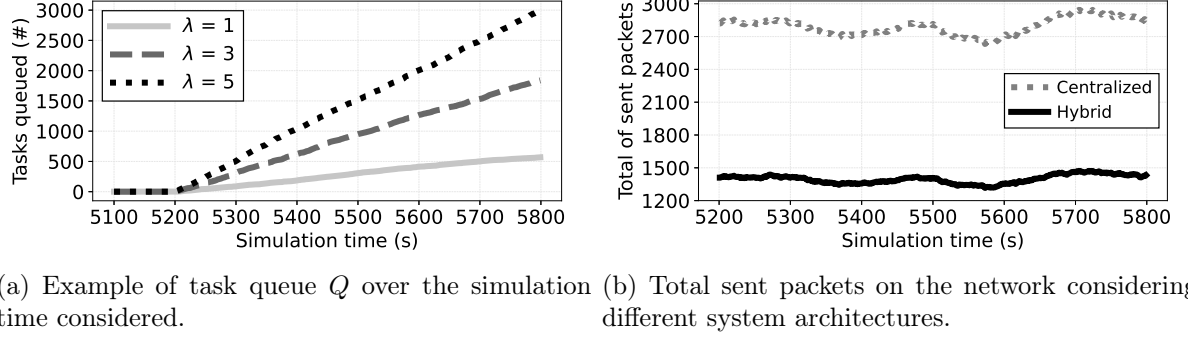
Figure 5.9: Task arrival rate example and total sent packets on the network.
