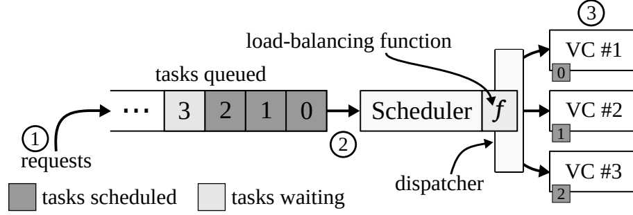
Figure 6.2: The task scheduling pipeline with a load-balancing function integrated into the scheduler.
