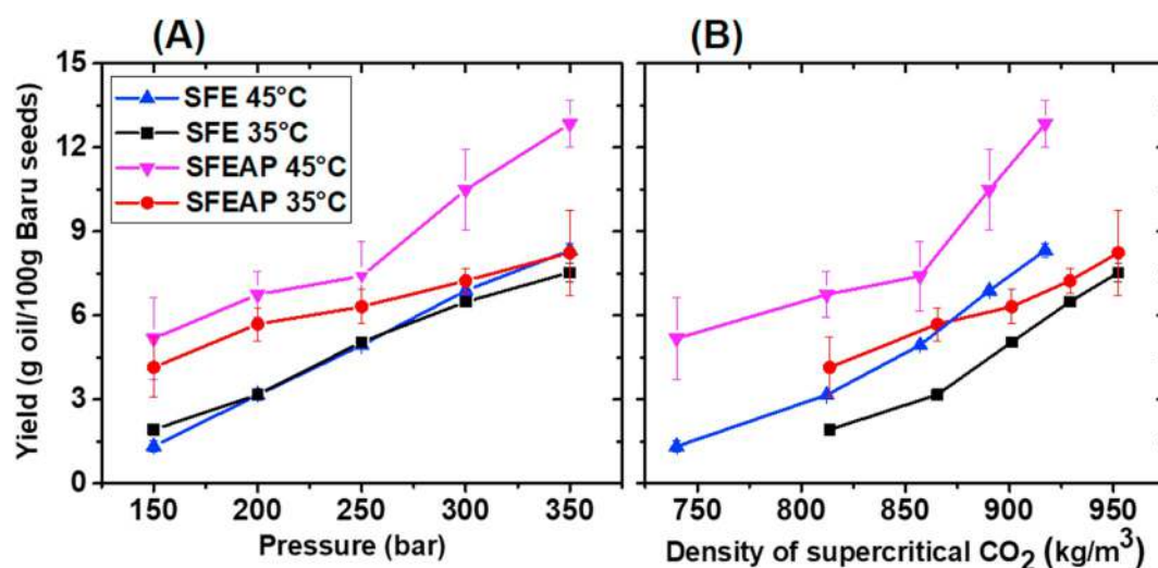
Figure 3. Extraction yield of Baru seed oil with sc-CO 2 at different pressures (150–350 bar). (A) and densities (740.05–952.25 kg m -3 ) (B), with (SFEAP) and without pressing (SFE) at 35 and 45 °C. The CO 2 flow rate was 7 g/min, and the S/F ratio was 12.
