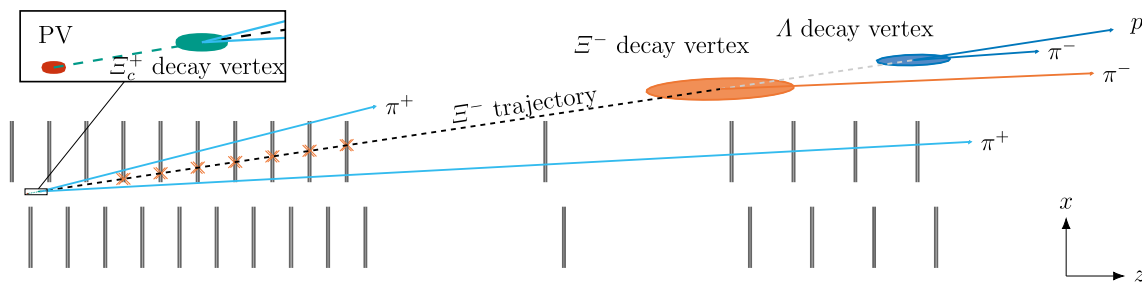
Fig. 3 Illustration of the E_c^+ \rightarrow E^- \pi^+ \pi^+ decay. The VELO modules are drawn as vertical gray lines; reconstructed final state particles as colored straight lines; trajectories of decaying particles as dashed lines;
