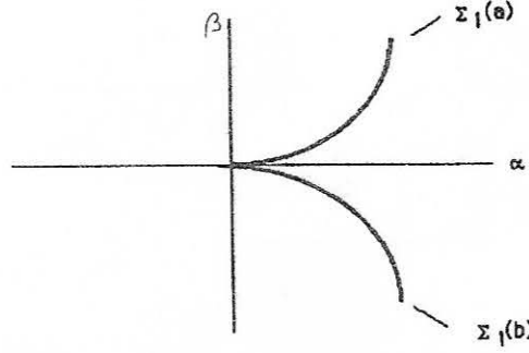
Figure 1: Bifurcation diagramm of a t_1 -singularity
