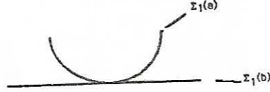
Figure 3: Bifurcation diagram of a t_2 -singularity
