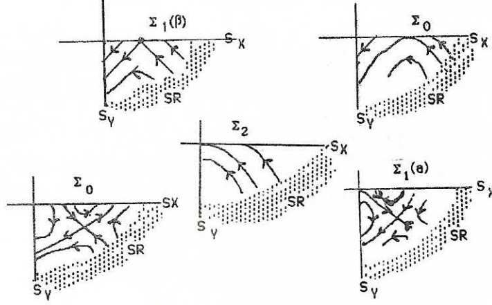
Figure 9: Unfolding of a t_4 -singularity
