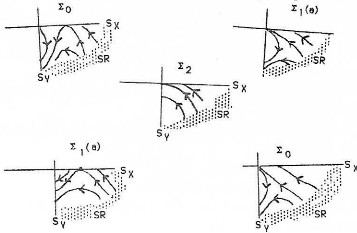
Figure 6: Unfolding of a t_3 -singularity
