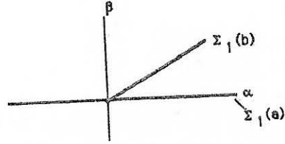
Figure 8: Bifurcation diagram of a t_4 -singularity
