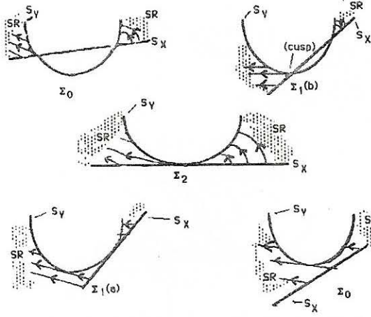
Figure 4: Unfolding of a t_2 -singularity
