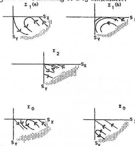
Figure 7: Unfolding of a t_3 -singularity (distinguished saddle case)
