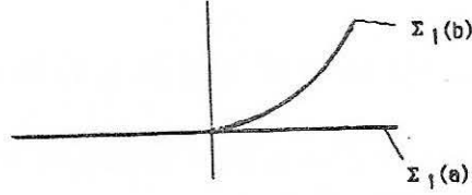
Figure 5: Bifurcation diagram of a t_3 -singularity (distinguished saddle case)
