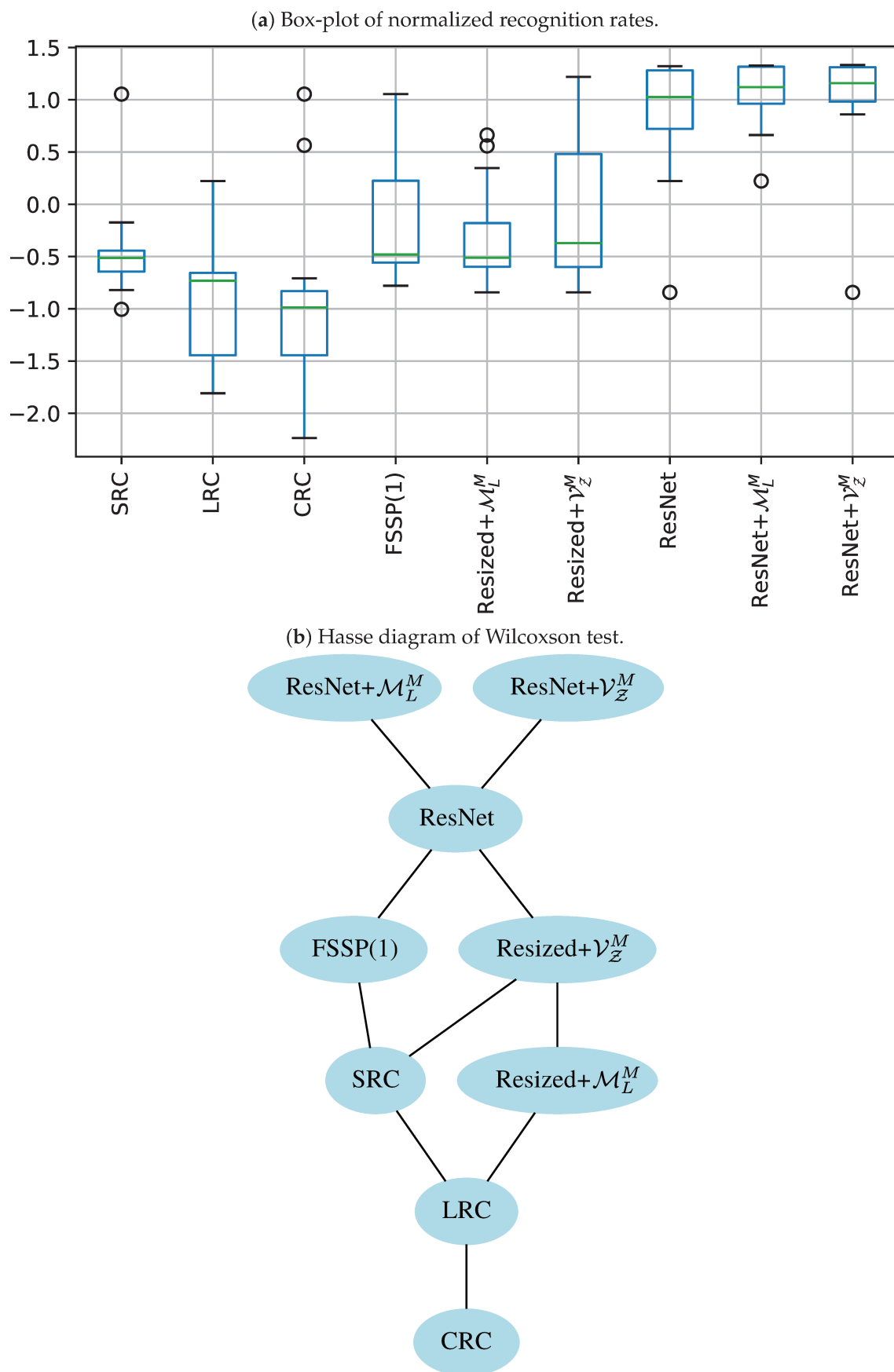
Figure 5. Box-plot and Hasse diagram of Wilcoxon signed-ranks test for the face recognition task.
