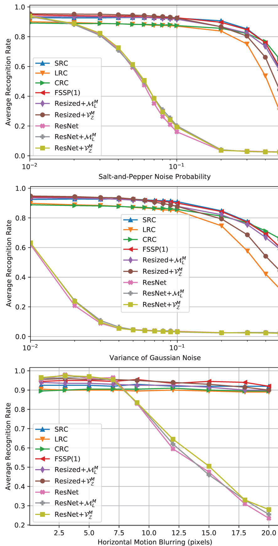
Figure 7. Average recognition rate (ARR) versus noise intensity or horizontal motion.
