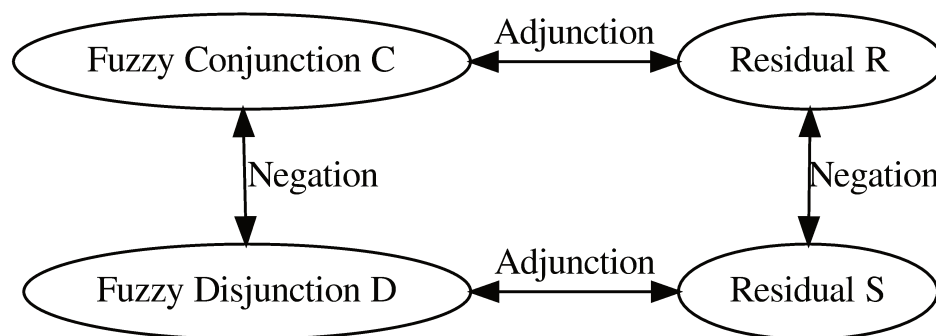
Figure 1. Relationship between fuzzy operations using adjunction and negation.
