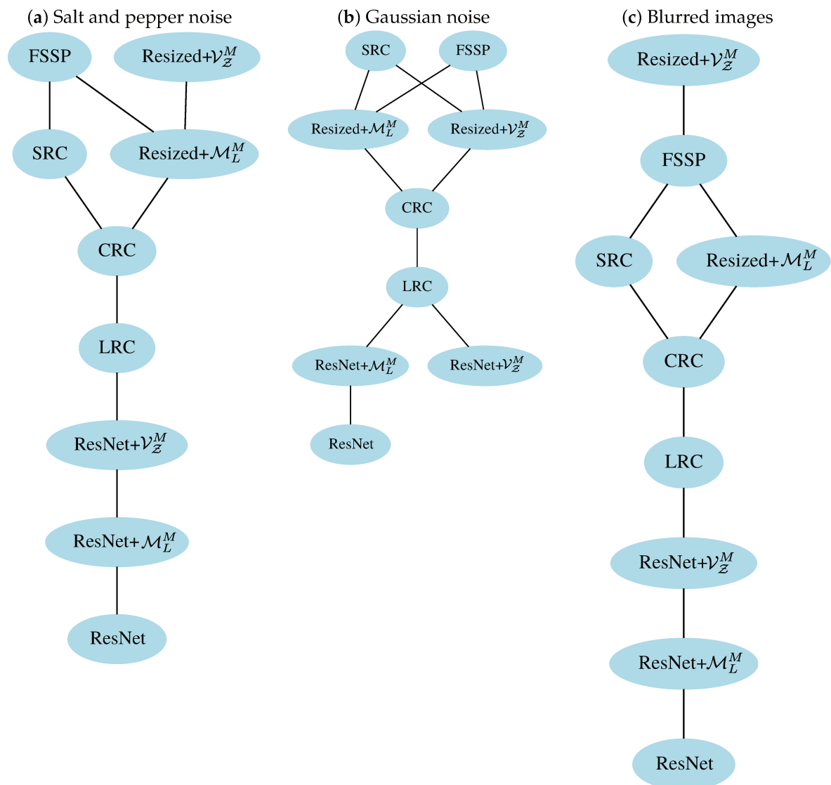
Figure 8. Hasse diagram of Wilcoxon signed-ranks test for the recognition task from corrupted input images.
