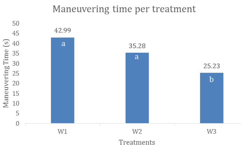
Figure 5. Comparison between means for the variable maneuvering time for treatments W1, W2, and W3.
