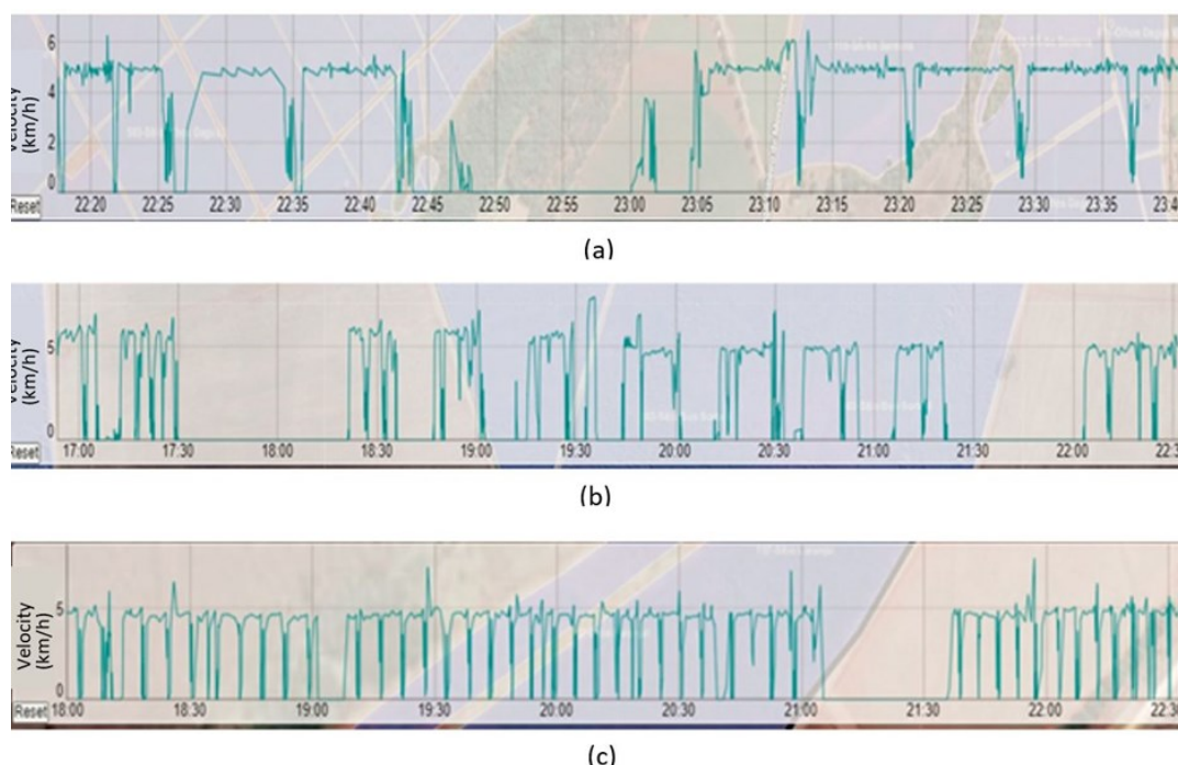
Figure 3. Speed variations as a function of the time for treatments W1 (a), W2 (b), and W3 (c).
