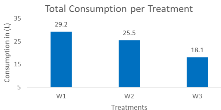
Figure 7. Total fuel consumption for treatments W1, W2, and W3
