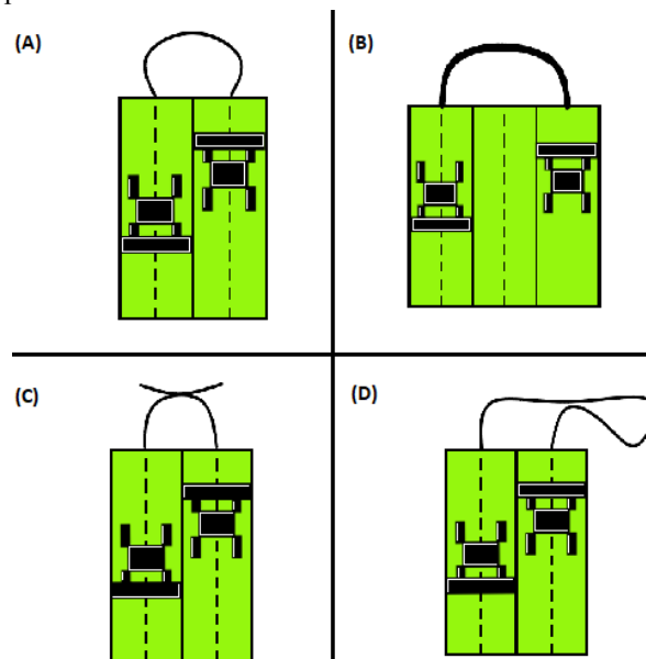
Figure 1 - Representation of the four types of maneuvers for realigning the harvester, namely: U (a), \Omega (b), P(c), and T(d). Source: elaborated by the authors
