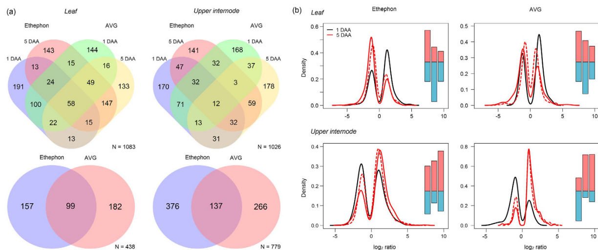
Figure 3. Overview of Sugarcane Assembled Sequences (SAS) identified as differentially expressed (DE) in sugarcane plants sprayed with ethephon and AVG after one and five days (DAA). (a) Venn diagrams for leaf and upper internode tissues using one-DAA (top) and five-DAA (bottom) mock samples as reference: N means the number of unique SAS in the diagram. (b) Density plots of log 2 ratio values (the bimodal distribution reflects the selection of DE SAS based on the HTself algorithm), including a bar chart with the number of up (red) and downregulated (blue) genes in the following order (left to right): one (black line) and five (red line) DAA chemical treated-samples against one DAA mock sample (solid line), and five DAA chemical treated-samples against five DAA mock sample (dashed line).
