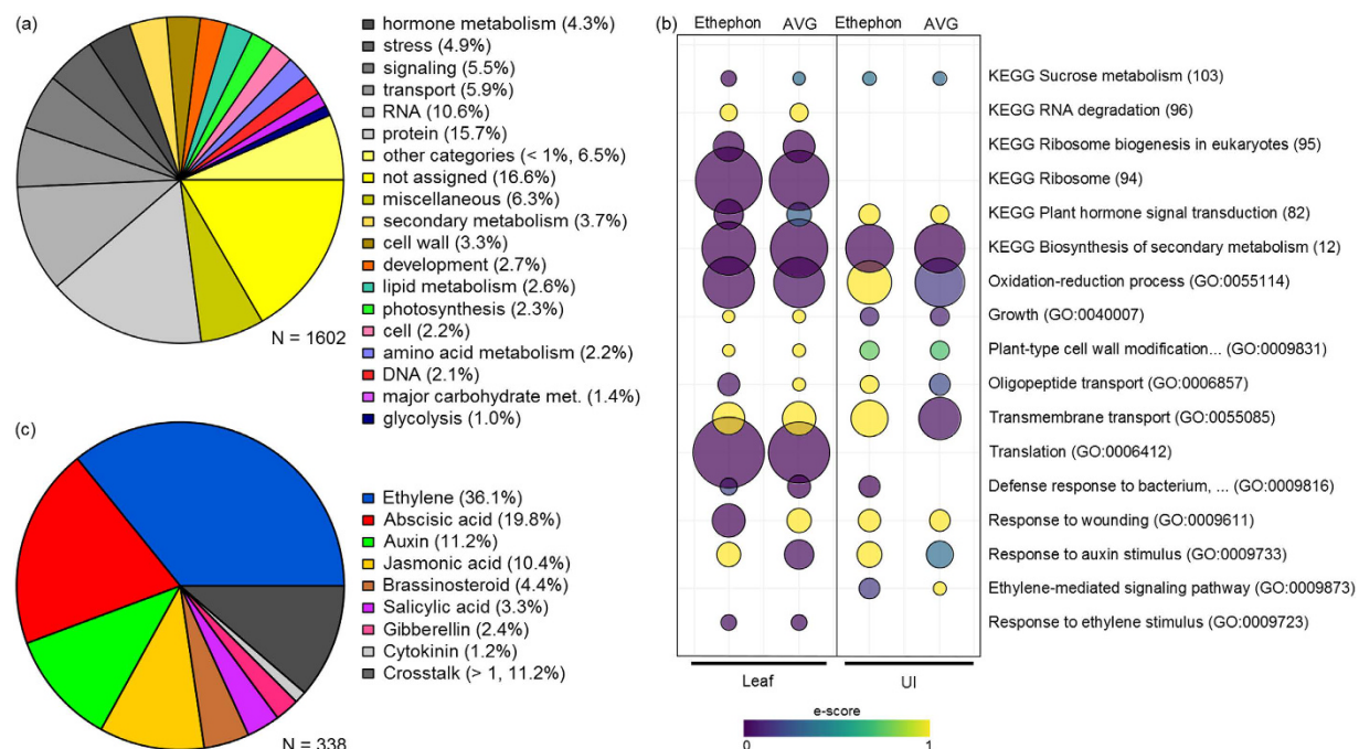
Figure 4. Functional enrichment analyses. (a) GOMapMan categories among Sugarcane Assembled Sequences (SAS) identified as differentially expressed (DE) with homology to Arabidopsis. (b) Selected statistically significant enriched GO (Gene Ontology) terms (biological process) and KEGG pathways identified in leaf and upper internode (UI) of plants sprayed with ethephon and AVG; the bubble size indicates the frequency of the GO term within the SAS set. (c) Proportion of hormone-related DE transcripts in each category.
