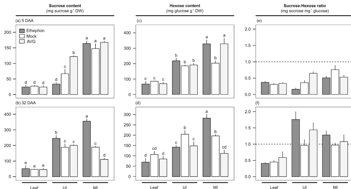
Figure 1. Sucrose (a,b) and hexose (reducing sugars, (c,d)) contents (mg sugar g -1 dry weight) and sucrose:hexose ratio (e,f) in leaf and upper (UI, immature) and middle (MI, maturing) internodes of sugarcane plants at five (a,c,e) and 32 (b,d,f) days after ethephon (dark gray), mock (white), or AVG (light gray) application (DAA). Each bar represents the average of four replicates (individual plants), including the standard error of the mean (SEM). The letters denote significant differences using two-way ANOVA (chemical versus tissue interaction, p -value < 0.05) followed by LSD test ( p -value < 0.05).
