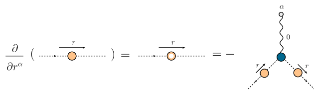
Fig. 7 Diagrammatic representation of the WI for the B\bar{c}c vertex, where the derivative of the ghost propagator can be identified as the insertion of a zero-momentum background gluon leg. Here we define the notation of a perforated circle as being the derivative acting on the Green's function
