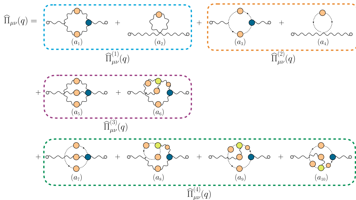
Fig. 1 Diagrammatic representation of the self-energy \hat{\Pi}_{\mu\nu}(q) . The small gray circles at the end of gluon legs indicate a background field. The orange and green circles represent conventional fully dressed prop-
