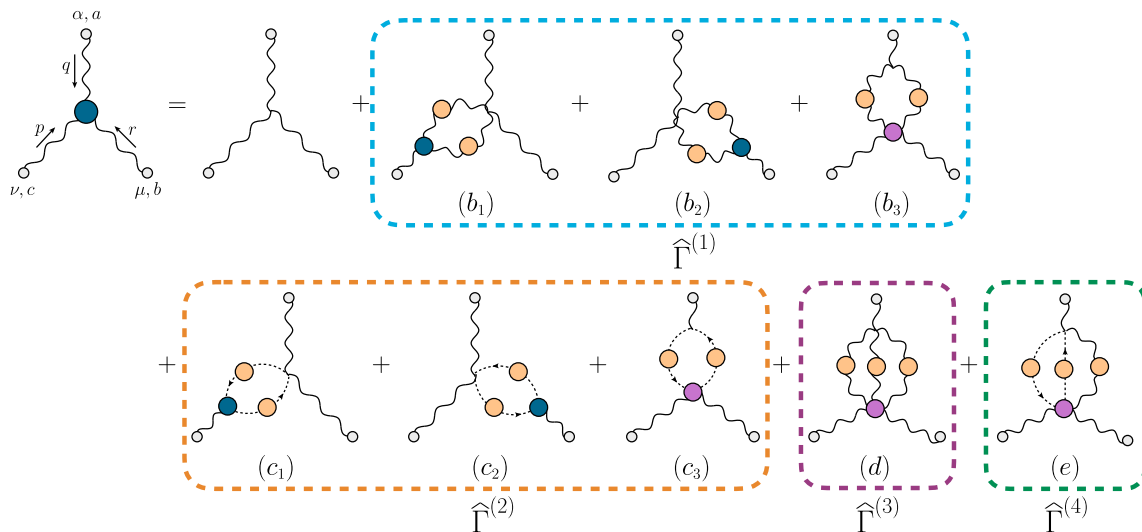
Fig. 2 The block-wise structure of the SDE which describes the three-gluon vertex \hat{\Gamma}_{\alpha\mu\nu}^{abc}(q, r, p) (BBB). The blue circles represent full one-particle irreducible vertices, while the purple ones the four- and five-point scattering kernels
