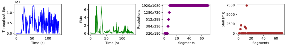
Figure 3.13: 4G: QoS interdependence with objective QoE – stall and quality shifts using Conventional – ABS and a window size of 1-second.
