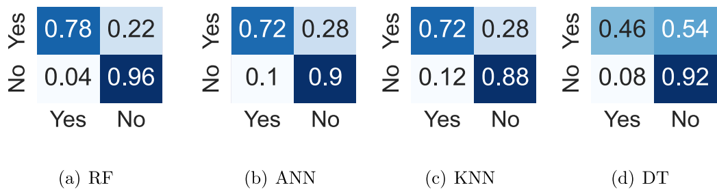
Figure 5.9: Confusion matrix 9s - RF, ANN, KNN and DT.
