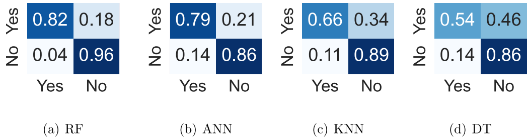
Figure 5.8: Confusion matrix 7s - RF, ANN, KNN and DT.
