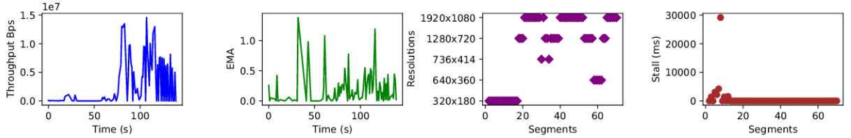
Figure 3.15: 5G: QoS interdependence with objective QoE – stall and quality shifts using Elastic – ABS and a window size of 1-second.
