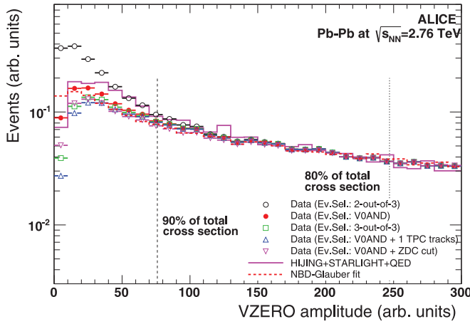
FIG. 12. (Color online) Distribution of the VZERO amplitude zoomed in the most peripheral region. The distribution is compared to the NBD-Glauber fit and to the sum of the HIJING + STARLIGHT + QED simulations.
