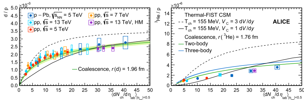
Fig. 5 Ratio between the p_T -integrated yields of nuclei and protons as a function of multiplicity for (anti)deutrons (left) and (anti)helions (right). Measurements are performed in INEL > 0 pp collisions at \sqrt{s} = 5.02 TeV, in high-multiplicity pp collisions at \sqrt{s} = 13 TeV [24], in INEL > 0 pp collisions at \sqrt{s} = 13 TeV [23, 24] and at \sqrt{s} = 7 TeV [6], and in p–Pb collisions at \sqrt{s_{NN}} = 5.02 TeV [11, 31]. The statistical uncertainties are represented by vertical bars while the systematic uncer-
