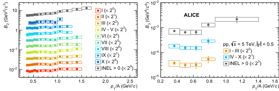
Fig. 3 Coalescence parameters B_2 for (anti)deutrons (left) and B_3 for (anti)helions (right) for different multiplicity classes. The multiplicity decreases moving from the bottom up. The statistical uncertainties are
