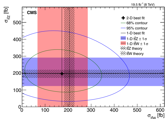
Fig. 5 The result of the two-dimensional best fit for t\bar{t}W and t\bar{t}Z cross sections (cross symbol) is shown along with its 68 and 95 % confidence level contours. The result of this fit is superimposed with the separate t\bar{t}W and t\bar{t}Z cross section measurements, and the corresponding 1 standard deviation ( 1\sigma ) bands, obtained from the dilepton, and the trilepton/four-lepton channels, respectively. The figure also shows the predictions from theory and the corresponding uncertainties
