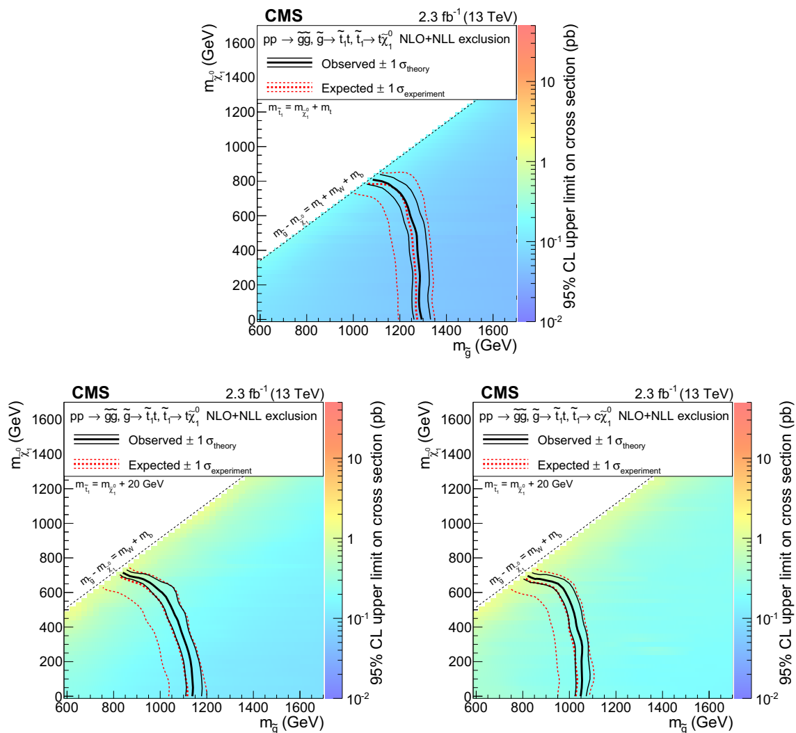
Fig. 5 Exclusion regions at the 95 % CL in the plane of m_{\tilde{\chi}_1^0} versus m_{\tilde{g}} for models with the gluino decaying to an on-shell top squark: T5tttt with m_{\tilde{\chi}_1^0} = m_{\tilde{\chi}_1^0} + m_t (top), T5tttt with m_{\tilde{\chi}_1^0} = m_{\tilde{\chi}_1^0} + 20 GeV (bot-
