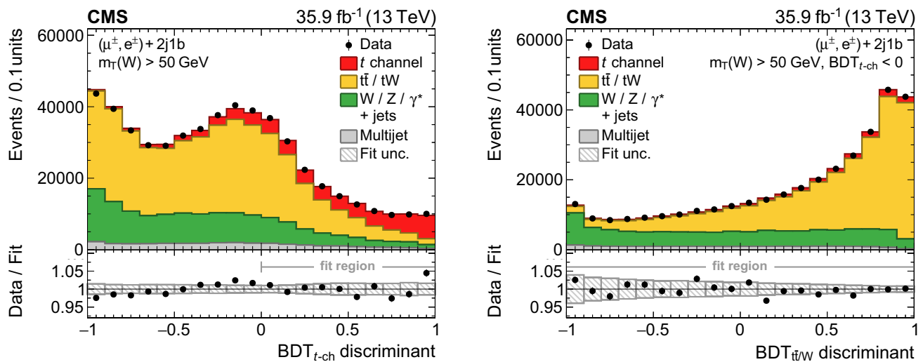
Fig. 3 Distributions of the BDT discriminants in the 2 jets, 1 b tag category: (left) BDT_{t-ch} trained to separate signal from background events; (right) BDT_{t\bar{t}/W} trained to separate t\bar{t} from W +jets events in a background-dominated category. Events in the muon and electron chan-
