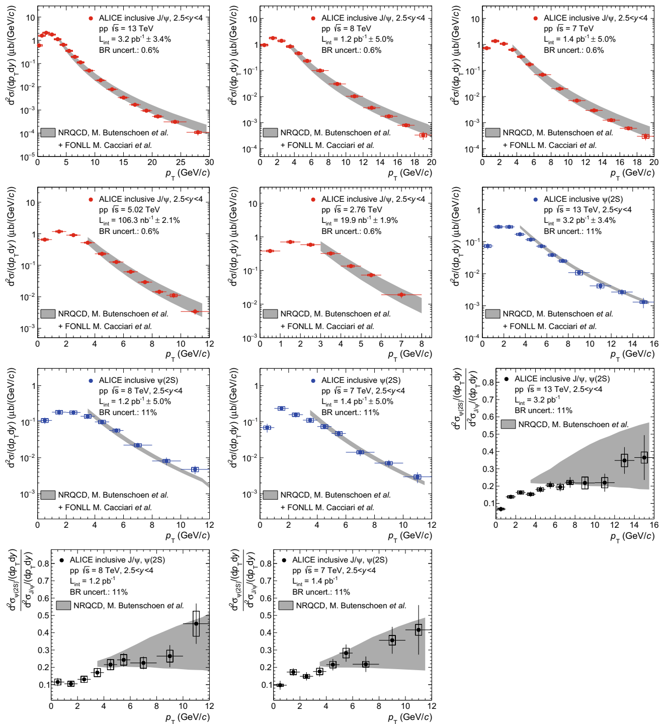
Fig. 10 Comparisons between ALICE J/ψ and ψ(2S) data and summed NRQCD and FONLL model calculations from [37,39]. The first five panels correspond to inclusive J/ψ production cross sections as a function of p_T in pp collisions at \sqrt{s} = 13, 8, 7, 5.02 and 2.76 TeV
