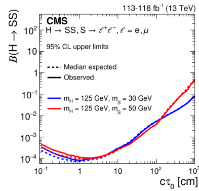
Fig. 6 The 95% CL upper limits on the H \rightarrow SS , S \rightarrow \ell^+\ell^- branching fraction as a function of c\tau_0 , for a Higgs boson with a mass of 125 GeV and a long-lived scalar with a mass of 30 GeV or 50 GeV, for the three channels combined. These limits assume that B(H \rightarrow SS) = 100\% and each S has a 50% probability of decaying to two electrons or two muons. The area above the solid (dashed) curve represents the observed (expected) exclusion region
