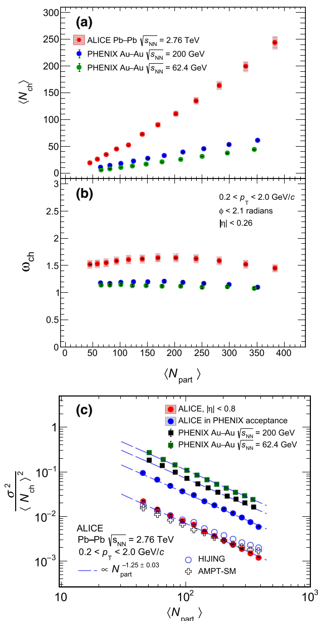
Fig. 3 Comparison of \langle N_{ch} \rangle , \omega_{ch} , and \sigma_{ch}^2/\langle N_{ch} \rangle^2 measured in this work based on the acceptance of the PHENIX experiment with results reported by PHENIX [31] as a function of number of participating nucleons, shown in panels a , b , and c , respectively. The statistical uncertainties are smaller than the size of the markers. The systematic uncertainties are presented as filled boxes
