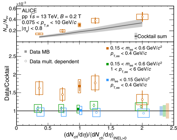
FIG. 3. Upper panel: Dielectron yield per event in the excess region as a function of the event multiplicity compared with the hadronic cocktail. Lower panel: Enhancement factor data or cocktail in three different kinematic regions. Error bars and boxes show the statistical and systematic uncertainties of the data points. The cocktail uncertainties are indicated as vertical bars around one in the lower panel.
