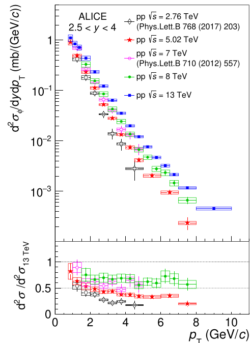
Fig. 3 Top: differential \phi meson production cross section d^2\sigma/(dy dp_T) as a function of p_T at \sqrt{s} = 2.76, 5.02, 7, 8 and 13 TeV. The boxes represent the systematic uncertainties, the error bars the statistical uncertainties. Bottom: ratio between the cross sections measured at several energies to the one obtained at \sqrt{s} = 13 TeV
