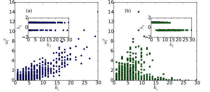
FIG. 6. (Color online). The graphics show the positive correlation between the magnitude of the natural frequencies and degrees for the optimized network to favor synchronization, panel (a), whereas there is no correlation for the network optimized to suppress synchronization, panel (b). Both results correspond to the networks depicted in figure 5. The insets show, for both cases, the distribution of the couplings as function of the degrees.
