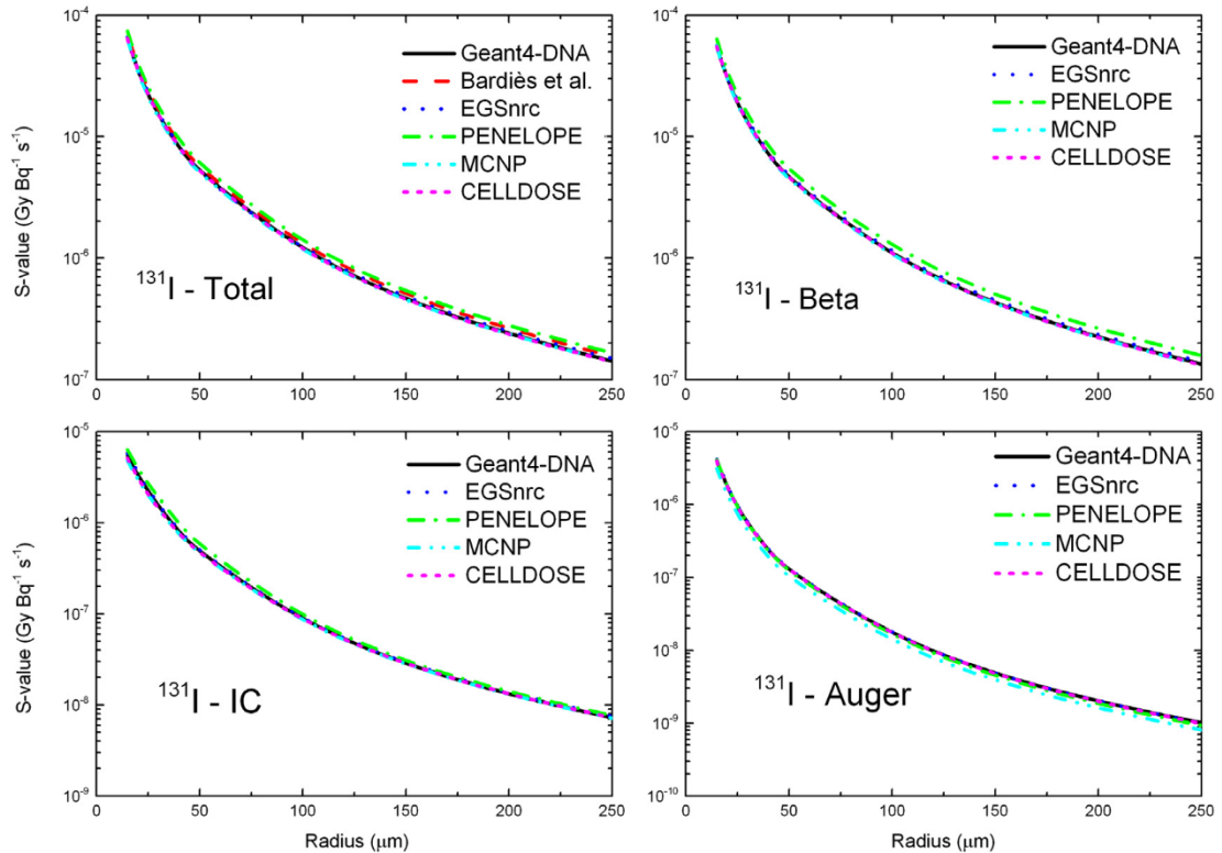
Fig. 3. Dependence of S-values obtained for 131 I as a function of colloid sphere radius, varying from 10 μm to 250 μm. Geant4-DNA results are compared to EGSnrc, CELLDOSE, MCNP and PENELOPE Monte Carlo codes and to Bardies and Chatal data [27]. S-values have been calculated for all processes (top-left), beta emission (top-right), internal conversion (bottom-left) and Auger emission (bottom-right).
