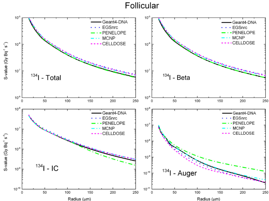
Fig. 4. Dependence of S -values obtained for ^{134}\text{I} as a function of follicular cells for radius varying from 10\text{ }\mu\text{m} to 250\text{ }\mu\text{m} . Geant4-DNA results are compared to EGSnrc, CELLDSE, MCNP and PENELOPE Monte Carlo codes. S -values have been calculated for all processes (top-left), beta emission (top-right), internal conversion (bottom-left) and Auger emission (bottom-right).
