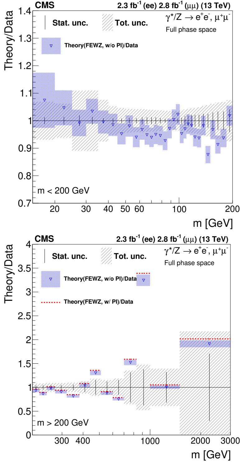
Figure 7. Magnified view of the ratio of the NNLO theoretical prediction of FEWZ with NNPDF 3.0 to data for the combined differential cross sections in two different mass ranges: m < 200 \text{ GeV} (top) and m > 200 \text{ GeV} (bottom). The blue bands represent the theoretical uncertainty on the ratio. The bottom plot also shows the ratio with the photon-induced contribution (red dashed lines), which has a sizable effect in the high-mass region.
