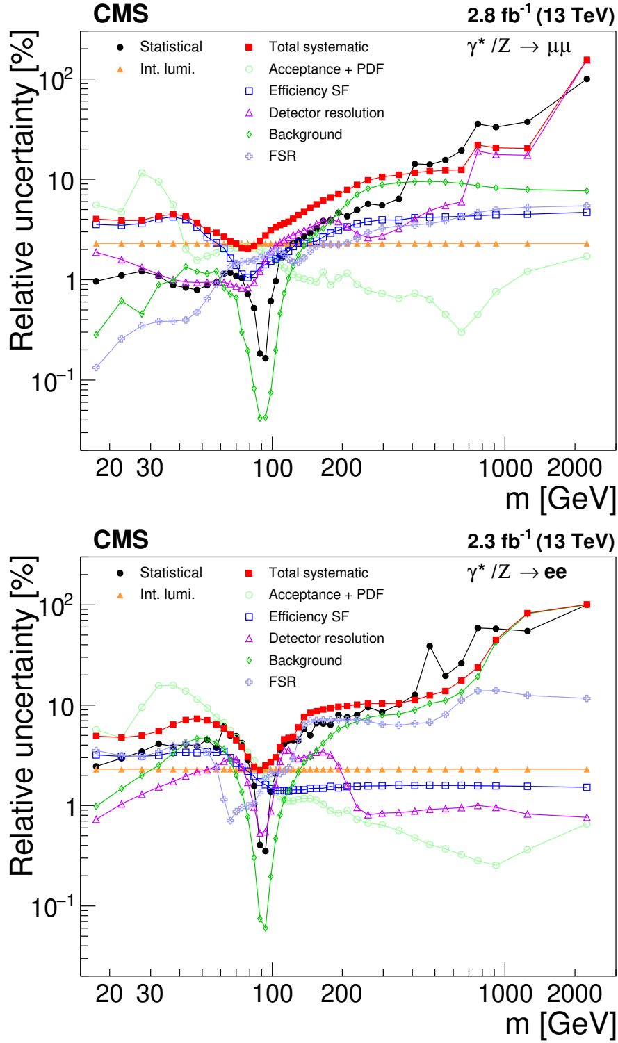
Figure 3. Summary of the systematic uncertainties on the differential cross section measurement d\sigma/dm [pb/GeV] in the dimuon (upper) and dielectron (lower) channels. The “Total systematic” is a quadratic sum of all systematic uncertainty sources except for the “Acceptance + PDF”.
