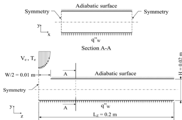
Figure 5. Duct configuration in two-dimensional confined jet.
