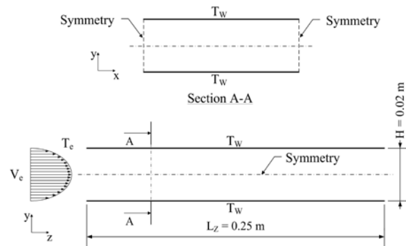
Figure 3. Dimensions and boundary conditions in channel flow.
