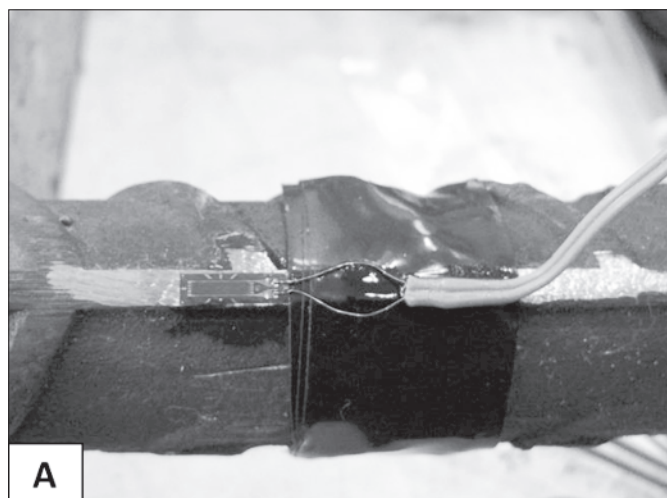
Figure 8 Detail of electrical extensometers: A - steel bar and B - coupler
