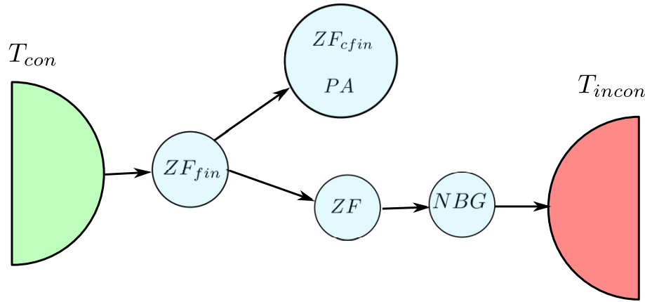
Figura 7 – Universo com PA(intF).
