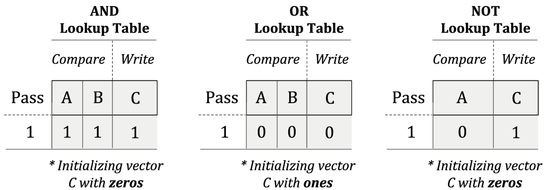
Figure 3.4: LUTs for AND, OR and NOT operations.
