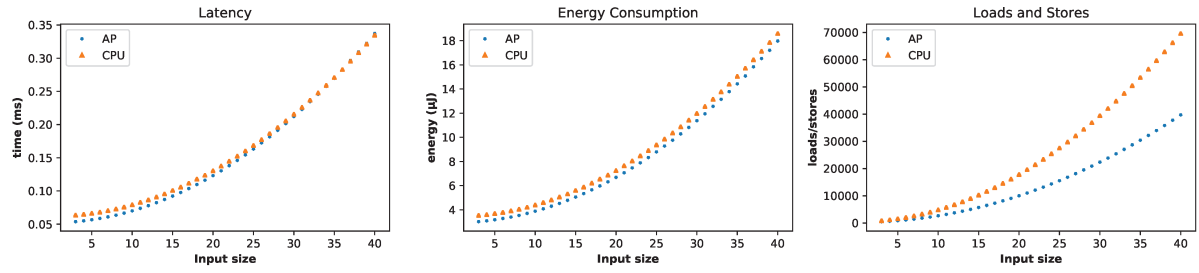
Figure 7.9: Latency, energy consumption and memory accesses for AP and CPU. The CPU performing optimized 2D convolution algorithm.
