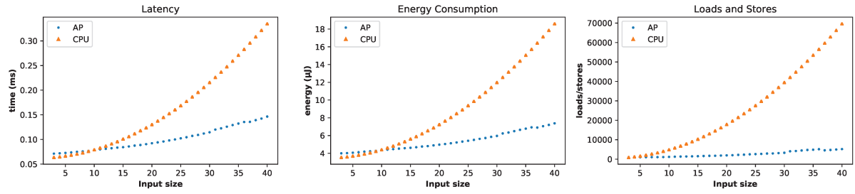
Figure 7.11: Latency, energy consumption and memory accesses for AP and CPU. The AP and CPU, both performing optimized 2D convolution algorithm.
