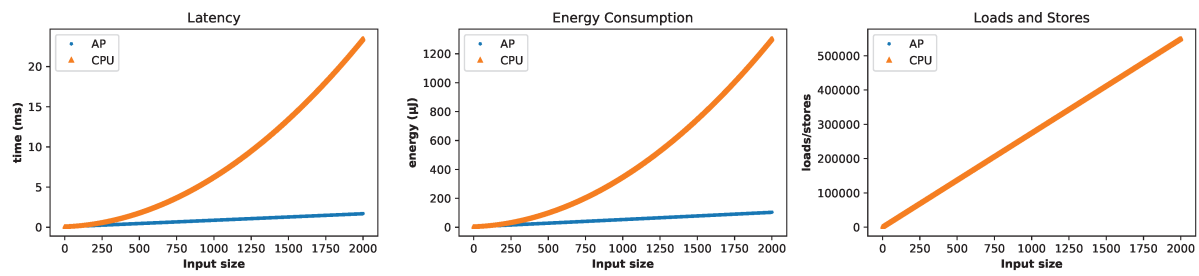
Figure 7.3: Latency, energy consumption and memory accesses for AP and CPU, both performing 1D convolution.
