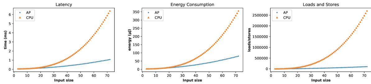
Figure 7.7: Latency, energy consumption and memory accesses for AP and CPU, both performing matrix multiply.
