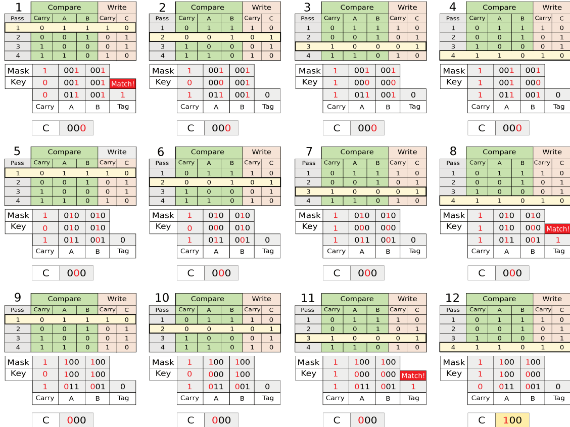
Figure 3.5: Associative ADD operation.
