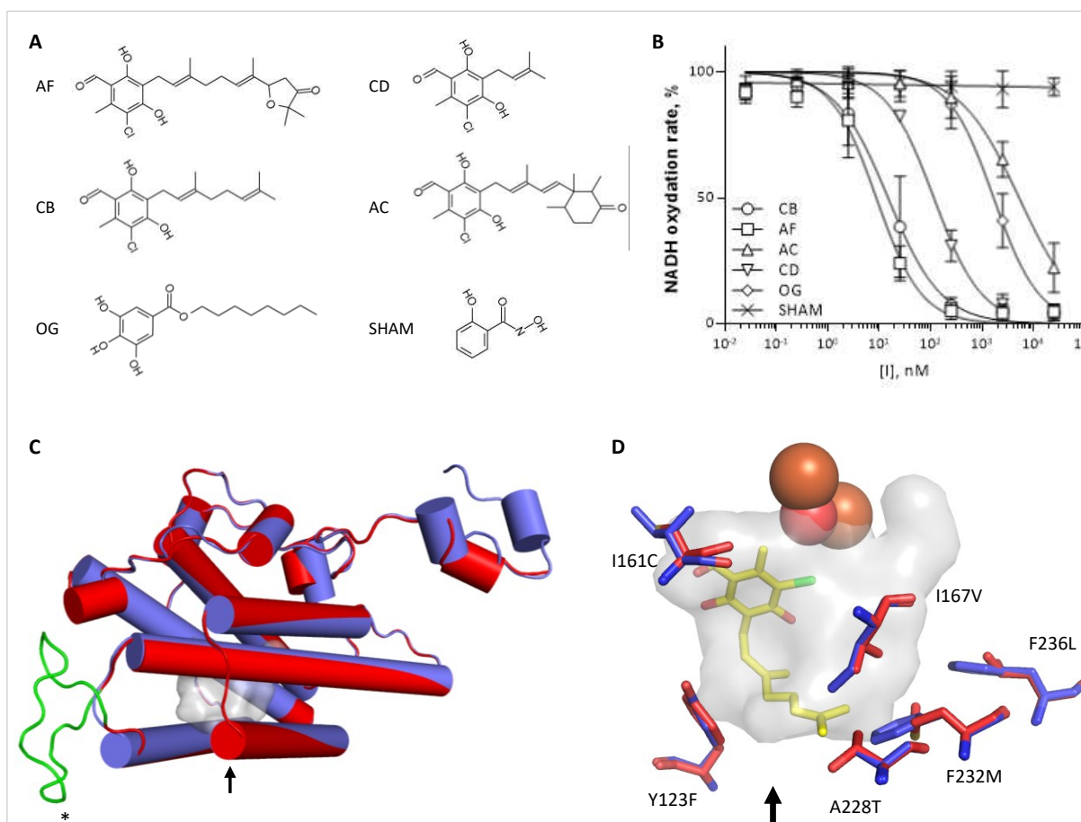
Fig. 2. Structure-activity relationship of MpAOX inhibitors. (A) Molecular structure of ascofuranone (AF), colletochorin D (CD), colletochlorin B (CB), ascochlorin (AC), octyl gallate (OG) and salicylhydroxamic acid (SHAM). (B) Dose-response assay with membrane-bound rMpAOX. Symbols represent the mean and standard deviation of three independent measurements. The continuous line is the best fit of a 4-parameter sigmoid function used to determine IC 50 values. (C) Overview of MpAOX (red; computer-generated) and TAO (blue; PBB ID 3w54) structures. The asterisk marks an insertion of 18 residues in MpAOX (green loop) found in fungal AOXs and likely necessary for activation by GMP. The arrow indicates the entrance to the substrate binding pocket (gray shading). (D) Analysis of MpAOX and TAO binding pocket composition. Amino acid residues that are different between those enzymes are shown as red (MpAOX) and blue (TAO) sticks, and listed in Table 1 . MpAOX residue numbering is used as reference. Yellow sticks depict CB present in the TAO crystal structure, and orange and red spheres represent two Fe 2+ and one OH - in TAO.
