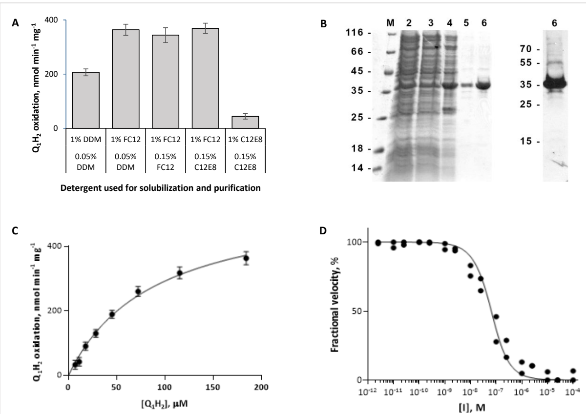
Fig. 3. Purification and kinetic characterization of rMpAOX. (A) Effect of detergents DDM, FC12 and C12E8 on pure rMpAOX activity. Each bar depicts the Q 1 H 2 oxidation rate of rMpAOX purified with the indicated detergents during membrane protein solubilization (top label) and affinity chromatography (bottom label). Membrane protein solubilization with FC12 allowed for the highest rMpAOX activity, regardless of the detergent employed in downstream steps. (B) Coomassie-brilliant blue-stained SDS-PAGE (left) and western blot (right) of protein samples collected during rMpAOX purification. M: molecular weight marker; 2: total E. coli protein; 3: clarified cell lysate; 4: E. coli membrane fraction; 5: affinity chromatography flow-through; 6: affinity chromatography eluate. (C) Kinetic characterization of rMpAOX with respect to ubiquinol-1 (Q 1 H 2 ). The assay was performed in 50 μL 20 mM tris-HCl buffer with 0.0125% C12E8 and 100 ng rMpAOX. The continuous line is the best fit for the Michaelis-Menten kinetic model. (D) Dose response assay with CB and 100 μM Q 1 H 2 . Points represent two independent measurements and the continuous line is the best fit for the Morrison equation [26].
