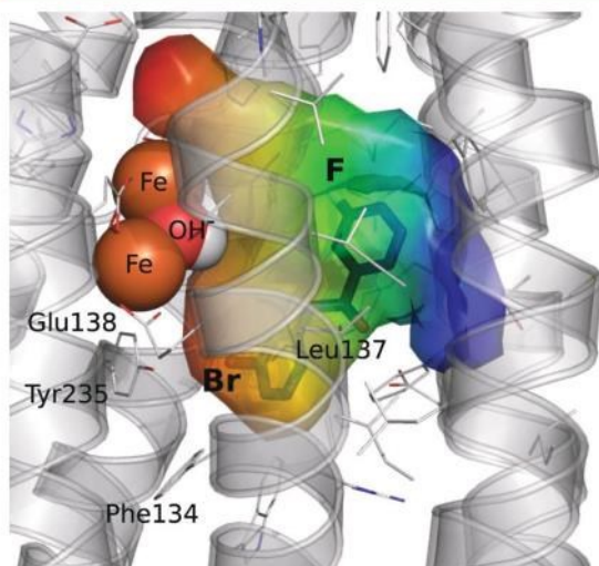
Figure 6. PpAOD structural model and docking of 7j-41. The best docking pose is shown. The color range represents from the aperture of the cavity to the solvent (blue) until the region farthest from that aperture (red). Residues Phe134, Leu137, Glu138 and Tyr235 make up the bromine interaction subsite.
