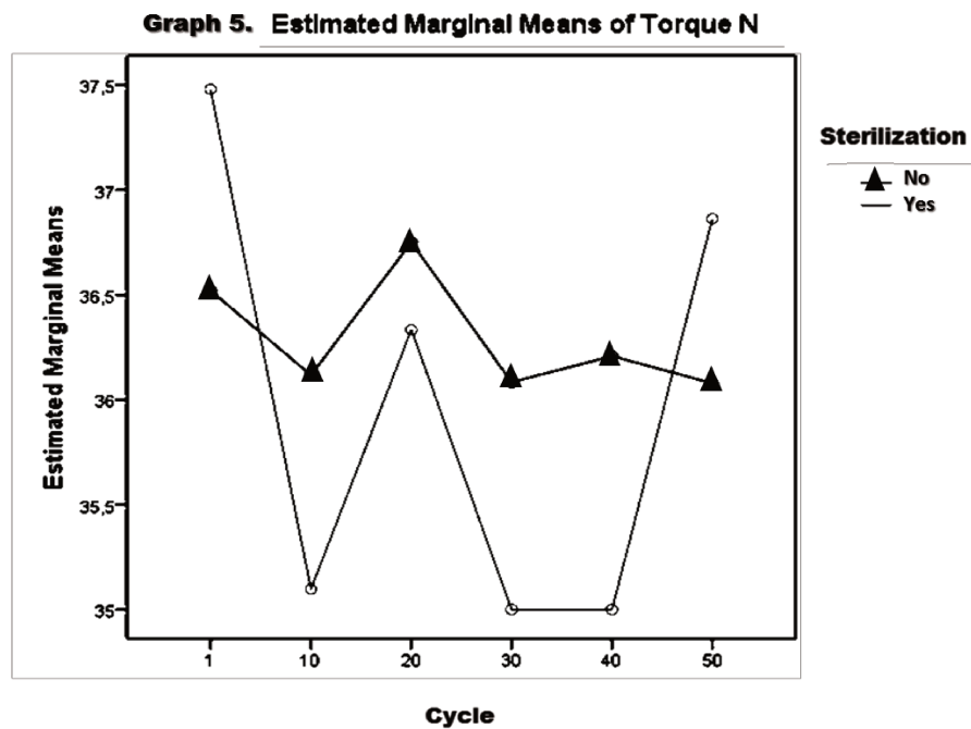
Graph 5. Comparative evaluation of the torque variation in the implant insertion in relation to the number of implants inserted (number of cycles) and the sterilization - Group III.
