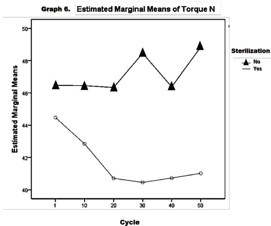
Graph 6. Comparative evaluation of the torque variation in the implant insertion in relation to the number of implants inserted (number of cycles) and the sterilization - Group II.
