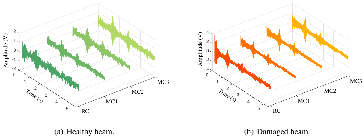
Figure 3.12 - Experimental control signals.
