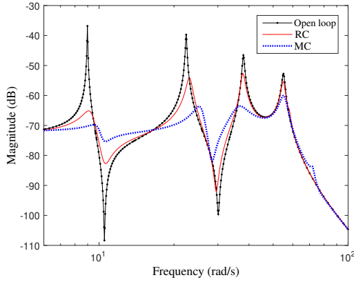
(a) T_{z_1 w} .
