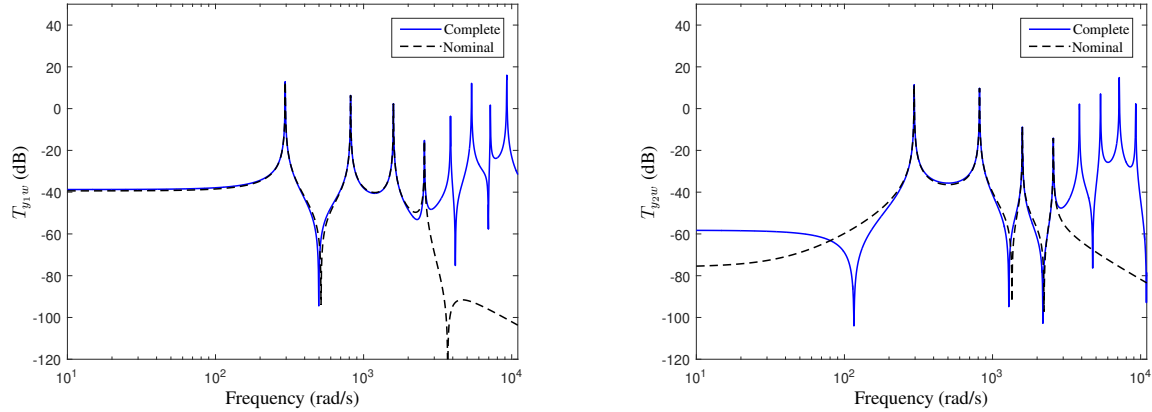
Figure 4.7 - Transfer function comparison between complete and nominal models.
