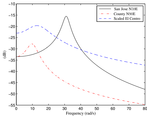
(a) Magnitude.
