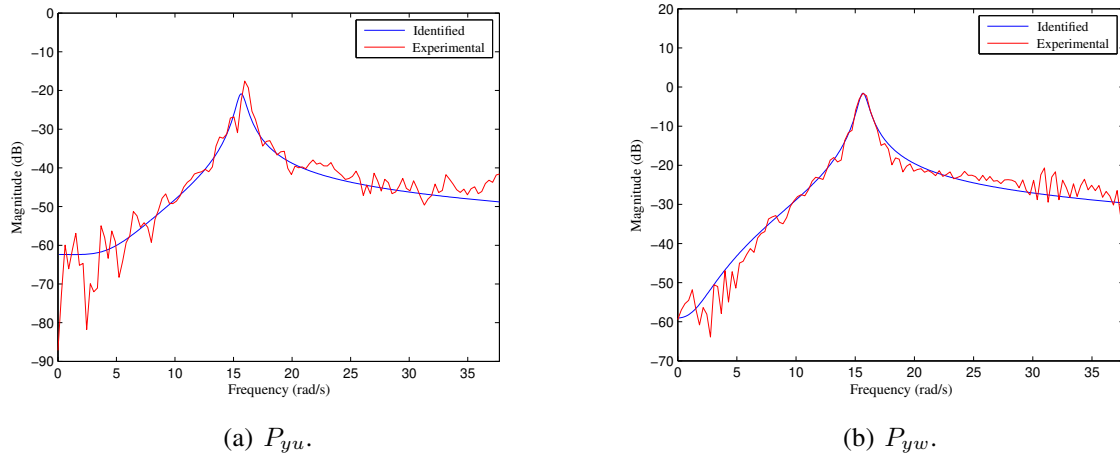
Figure 2.6 - Identified model.
