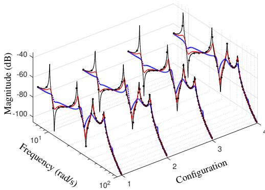
(a) T_{z_1 w} .
