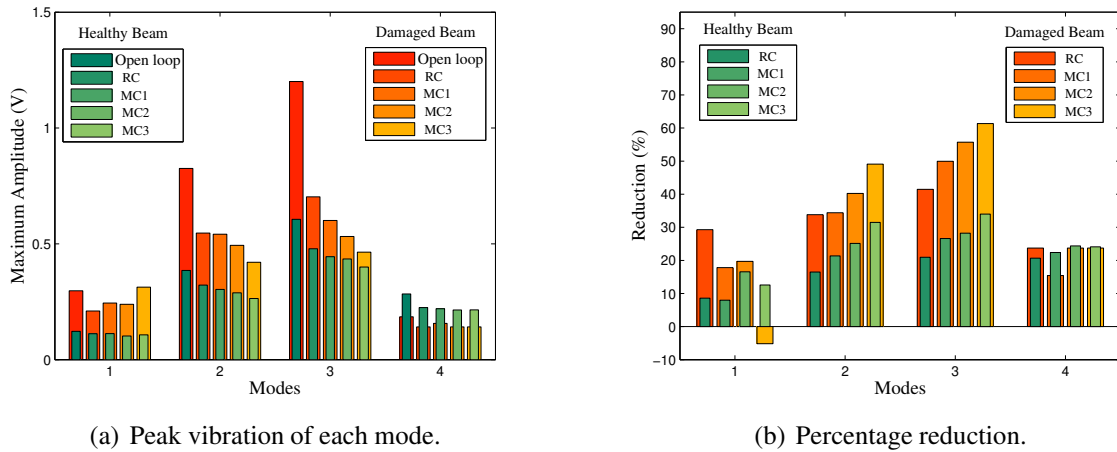
Figure 3.11 - Experimental output signals.
