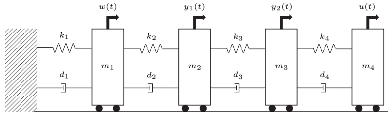
Figure 3.2 - Simulated structure.
