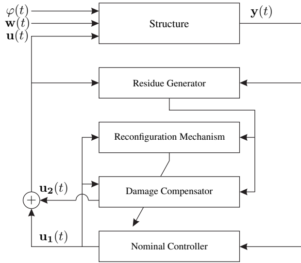
Figure 5.4 - Proposed DTAC framework.
