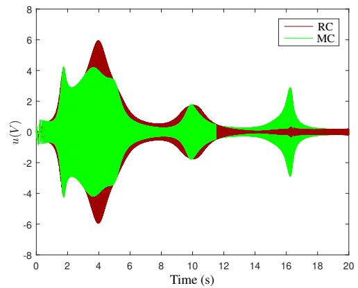
(b) Structure submitted to damage 2.
