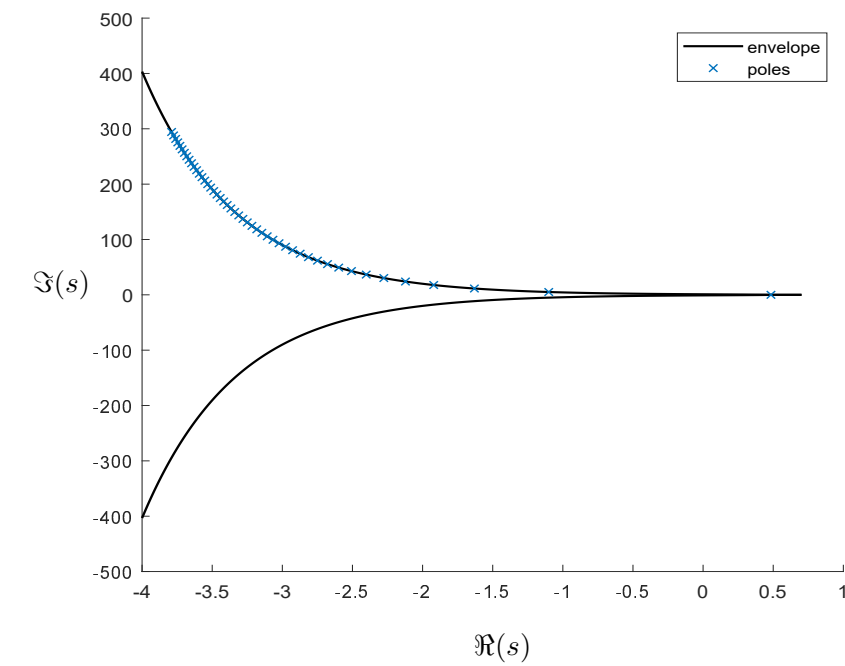
Figure 3.8: Stability Envelope for Fractional Retarded Time-Delay System
