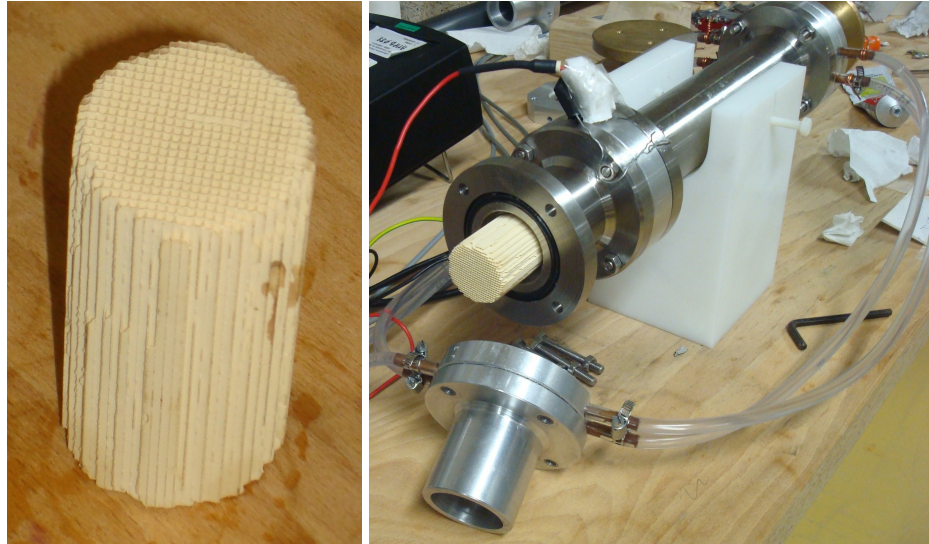
Figure 3.5: Ceramic Catalyst in detail and partially inserted in the open TAC.
