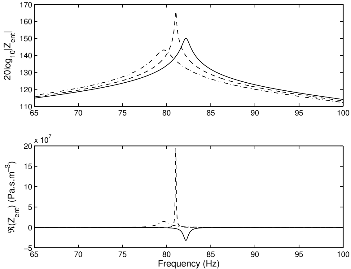
Figure 4.2: Ceramic Catalyst: modulus and real part of the reflected acoustic impedance for Q_H = 9\text{ W} (dash-dotted line), Q_H = 18\text{ W} (dashed line), and Q_H = 27\text{ W} (solid line).
