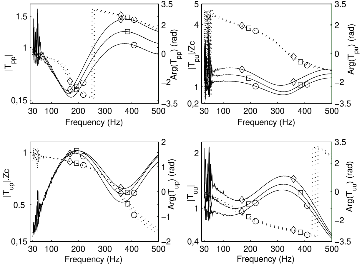
Figure 3.37: RVC Foam: amplitude (solid line) and phase (dotted line) of the T_{TAC} coefficients in the frequency domain for Q_H = 0 W (circle), Q_H = 9 W (square) and Q_H = 18 W (diamond) - Impedance Method.
