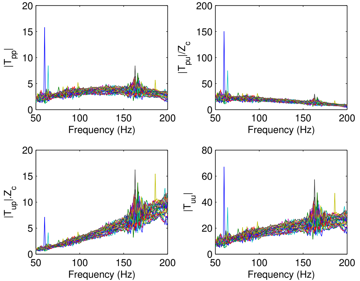
Figure D.3: Stainless Steel Grids: amplitude of the four T coefficients in the frequency domain for Q_H ranging from 0W to 81W , by a constant increment of 3W . - Two-Load Method.
