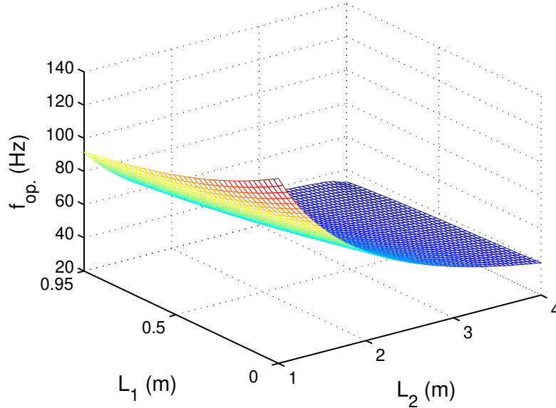
Figure 4.9: f_{op.} for closed-loop engines at Q_H = 81 W from measured \mathbf{T}_{TAC} of the Nichrome Foam using polynomial regression of fifth degree - Impedance Method.
