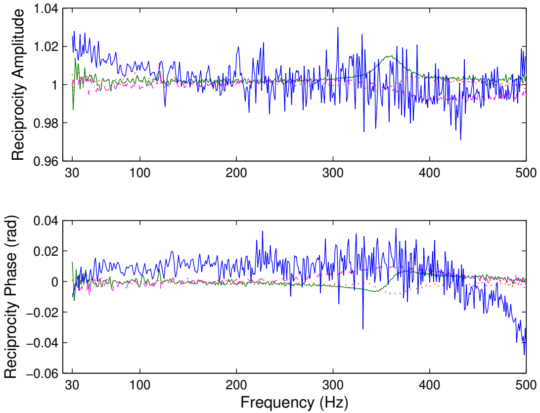
Figure 3.38: Amplitude and phase of the \mathbf{T}_{\text{TAC}} reciprocity in the frequency domain for Q_H = 0 W for the Stainless Steel Grids (relatively noisy lines), Ceramic Catalyst (continuous thin lines), Nichrome Foam (dotted lines) and RVC Foam (dashed lines) - Impedance Method.
