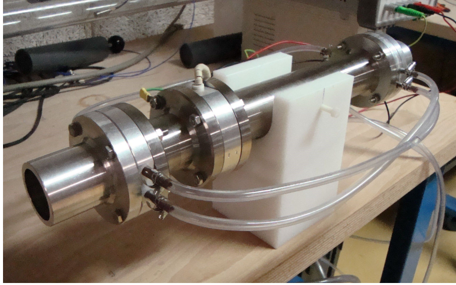
Figure 3.2: ThermoAcoustic Core.
