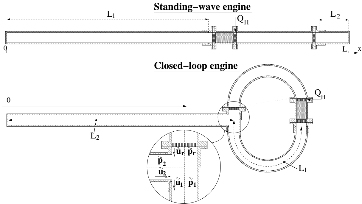
Figure 4.1: Basic configurations for standing-wave and closed-loop engines.
