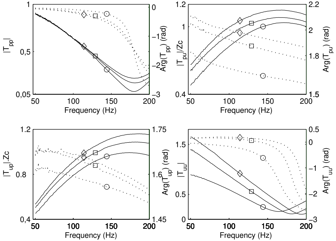
Figure 3.7: Ceramic Catalyst 1: amplitude (solid line) and phase (dotted line) of the \mathbf{T}_{\text{TAC}} coefficients in the frequency domain for Q_H = 0\text{ W} (circle), Q_H = 36\text{ W} (square) and Q_H = 72\text{ W} (diamond) - Two-Load Method.
