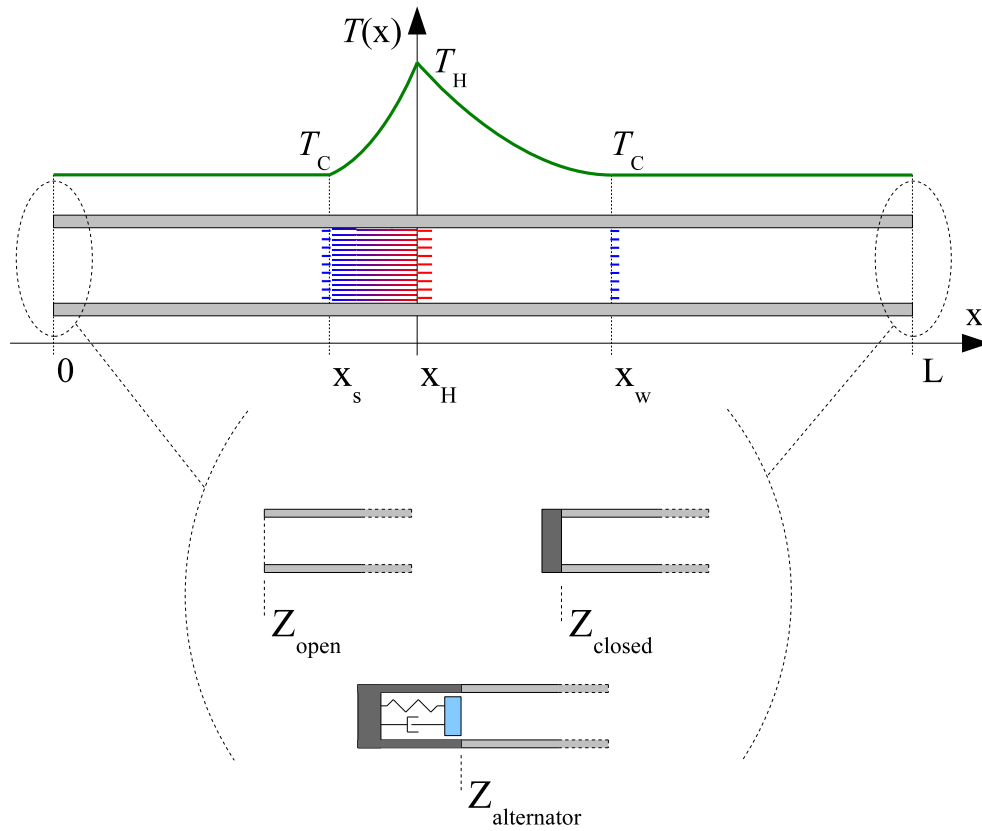
Figure 2.3: (a) Sketch of a standing-wave thermoacoustic engine. (b) Open end. (c) Closed end. (d) Coupling with an electrodynamic alternator.
