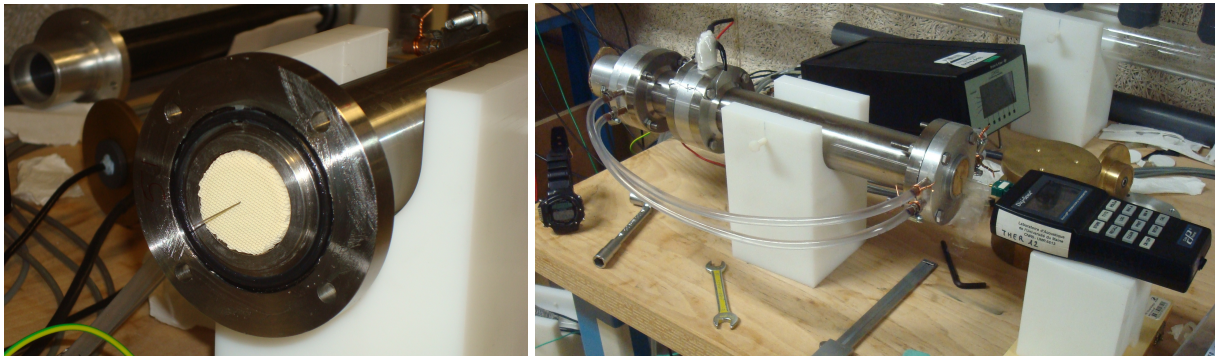
Figure 3.33: Temperature measurements at the right side of the HHX by means of a 35\text{ cm} long thermocouple accessing it from the TAC right side; the RVC Foam is within the TAC.
