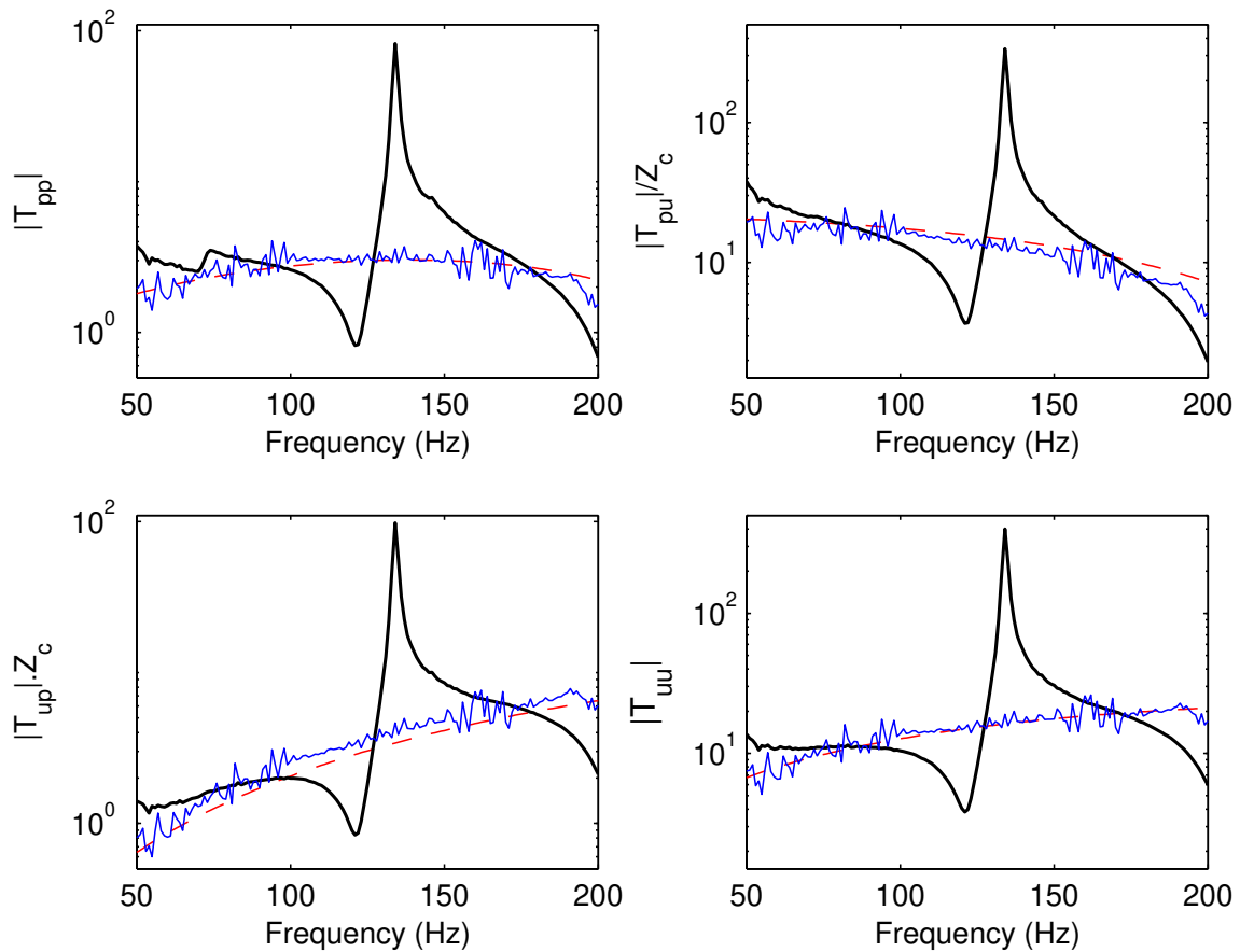
Figure 3.11: Stainless Steel Grids: amplitude of the \mathbf{T}_{\text{TAC}} coefficients in the frequency domain for Q_H = 0\text{ W} - Two-Load Method with TAC Inversion (bold lines), Two-Load Method (thin lines) and Theory (dashed lines).
