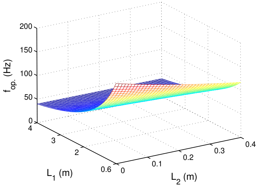
Figure 4.7: f_{op.} for standing-wave engines at Q_H = 81 W from measured \mathbf{T}_{TAC} of the Ceramic Catalyst using polynomial regression of fifth degree - Impedance Method.
