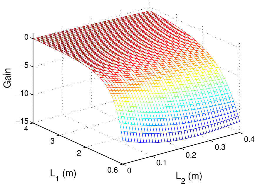
Figure 4.6: Gain for standing-wave engines at Q_H = 0 W from measured T_{TAC} of the Ceramic Catalyst using polynomial regression of fifth degree - Impedance Method.
