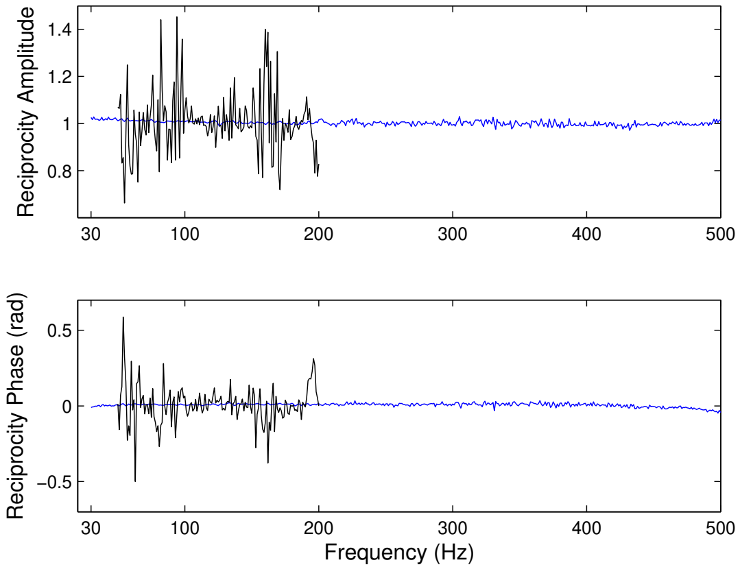
Figure 3.39: Stainless Steel Grids: amplitude and phase of the \mathbf{T}_{TAC} reciprocity in the frequency domain for Q_H = 0 W for the Impedance Method and for the Two-Load Method (very noisy lines).
