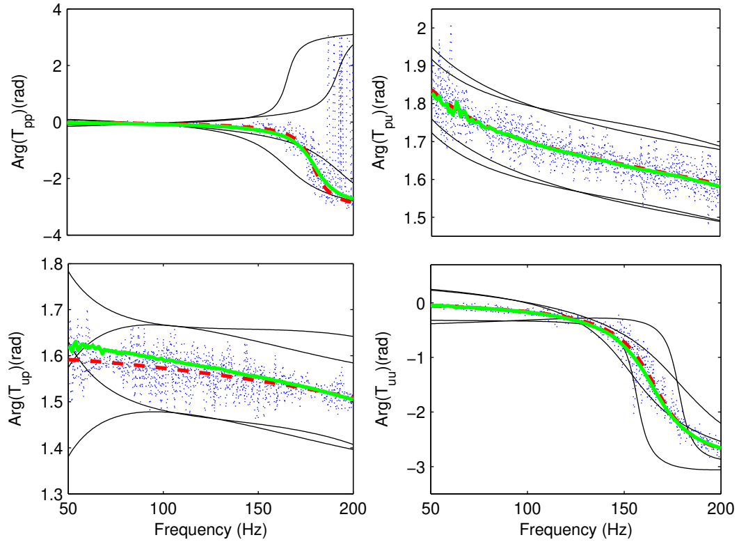
Figure 3.16: Ceramic Catalyst: phase of the four \mathcal{T} coefficients in the frequency domain for Q_H = 0 W in bold lines for the measurements (solid) and theory (dashed) with the respective theoretical bias (four thin solid lines per graph) and noise (five dotted lines per graph). - Two-Load Method.
