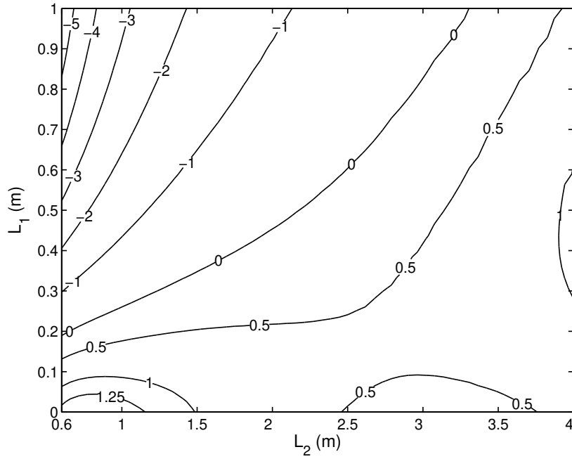
Figure 4.13: Gain for closed-loop engines at Q_H = 81 W from measured T_{TAC} of the Ceramic Catalyst using polynomial regression of fifth degree - Impedance Method.
