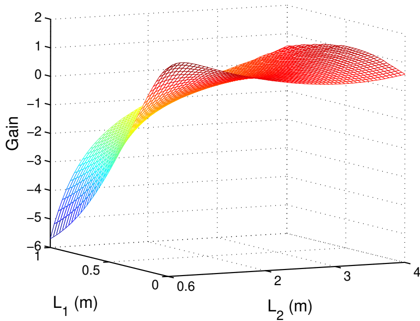
Figure 4.12: Gain for closed-loop engines at Q_H = 81\text{ W} from measured T_{TAC} of the Ceramic Catalyst using polynomial regression of fifth degree - Impedance Method.
