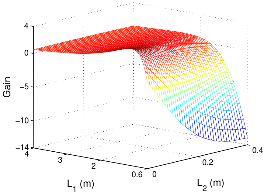
Figure 4.8: Gain for standing-wave engines at Q_H = 81 W from measured T_{TAC} of the Ceramic Catalyst using polynomial regression of fifth degree - Impedance Method.
