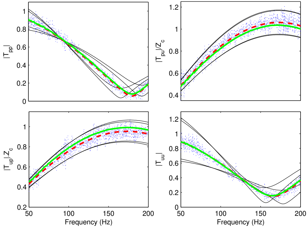
Figure 3.15: Ceramic Catalyst: amplitude of the four \mathcal{T} coefficients in the frequency domain for Q_H = 0W in bold lines for the measurements (solid) and theory (dashed) with the respective theoretical bias (four thin solid lines per graph) and noise (five dotted lines per graph). - Two-Load Method.
