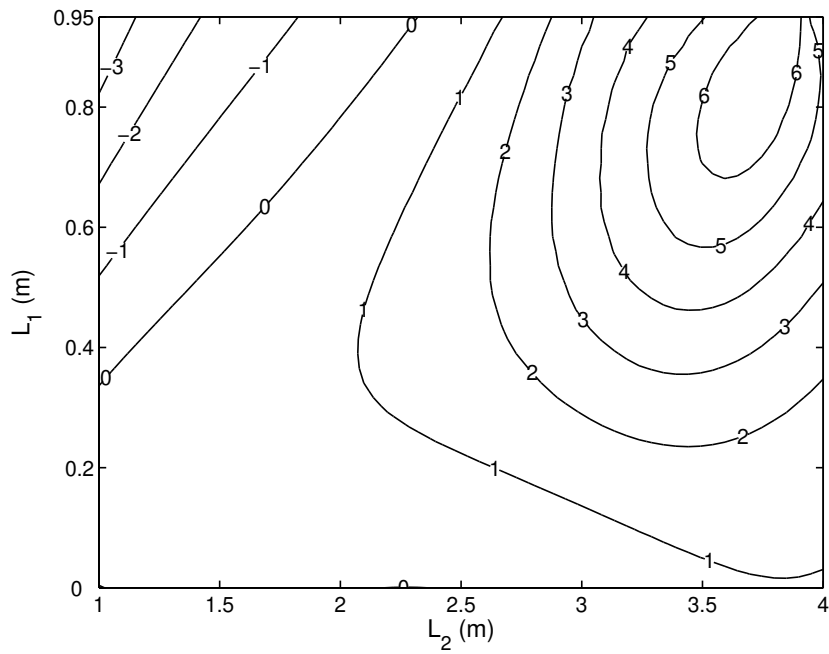
Figure 4.11: Gain for closed-loop engines at Q_H = 81\text{ W} from measured T_{TAC} of the Nichrome Foam using polynomial regression of fifth degree - Impedance Method.
