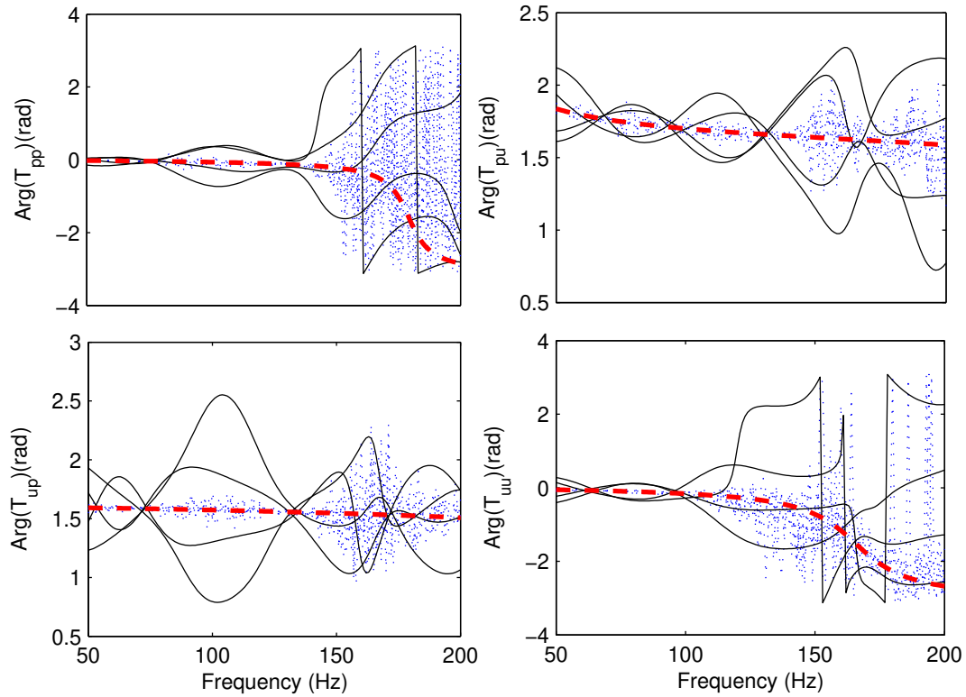
Figure 3.18: Ceramic Catalyst: phase of the four \mathcal{T} coefficients in the frequency domain for Q_H = 0 W in bold lines for the theory (dashed) with the respective theoretical bias (four thin solid lines per graph) and noise (five dotted lines per graph). - Two-Load Method with TAC Inversion.
