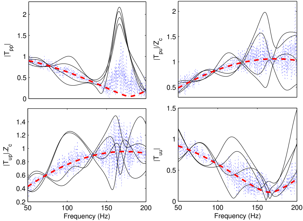
Figure 3.17: Ceramic Catalyst: amplitude of the four \mathcal{T} coefficients in the frequency domain for Q_H = 0W in bold lines for the theory (dashed) with the respective theoretical bias (four thin solid lines per graph) and noise (five dotted lines per graph). - Two-Load Method with TAC Inversion.
