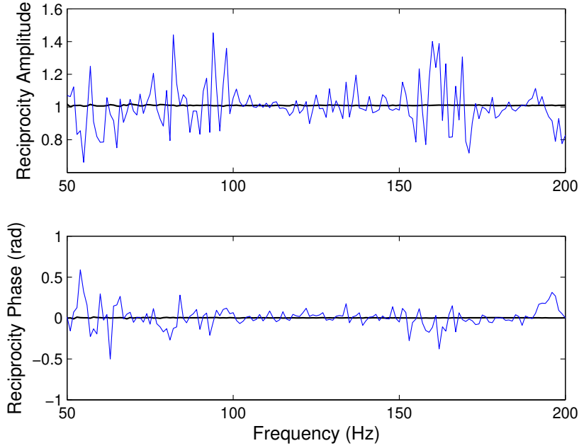
Figure 3.8: Amplitude and phase of the \mathbf{T}_{\text{TAC}} reciprocity in the frequency domain for Q_H = 0 W for the Ceramic Catalyst 600 cpsi (bold lines) and the Stainless Steel Grids (thin lines)- Two-Load Method.
