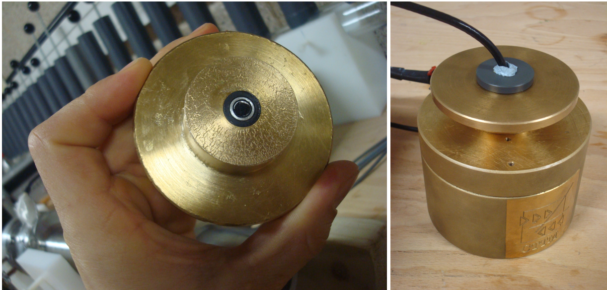
Figure C.1: Detail of the third microphone head and its attachment to the AIS for calibration.
