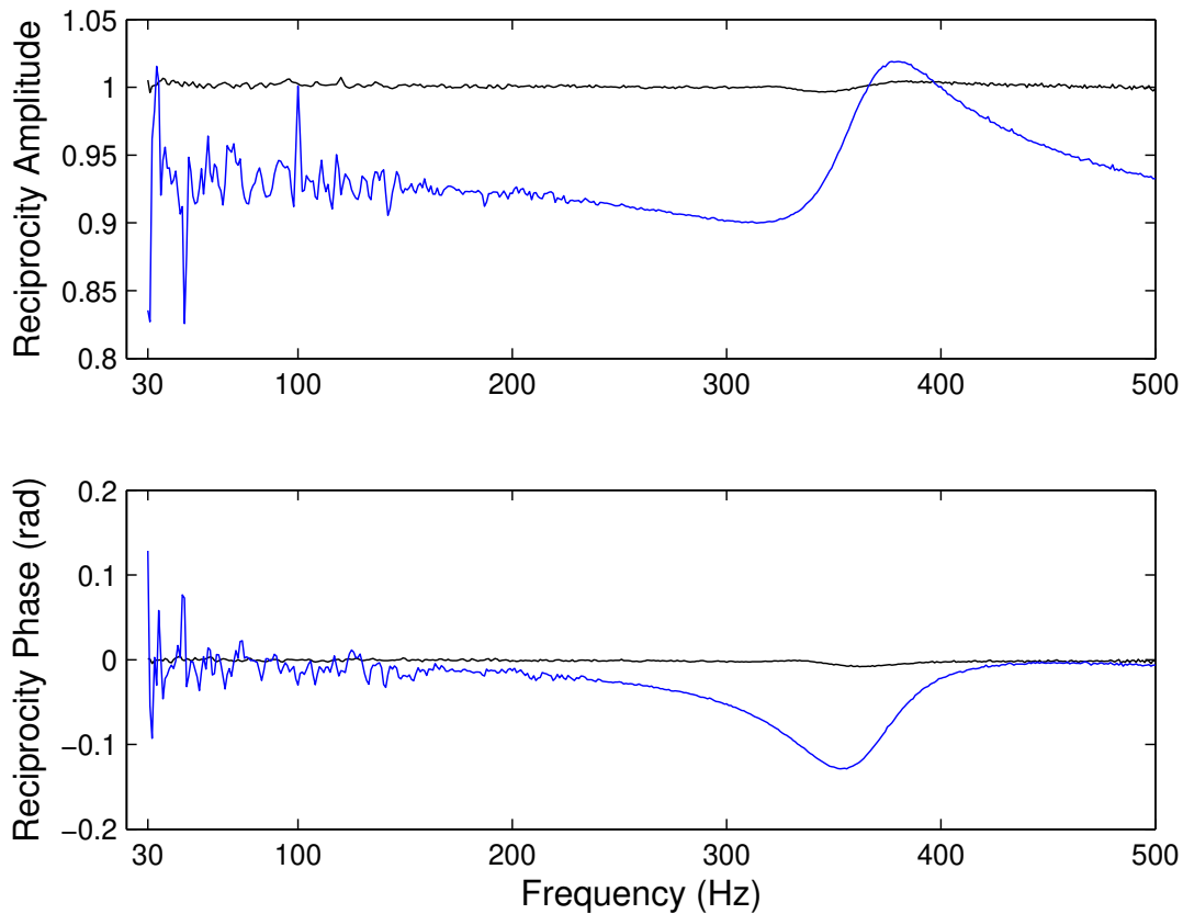
Figure E.1: NiCr Foam: amplitude and phase of the \mathbf{T}_{TAC} reciprocity in the frequency domain for Q_H = 0\text{ W} for the Impedance Method before (biased and noisy line) and after a better thermal stabilization.
