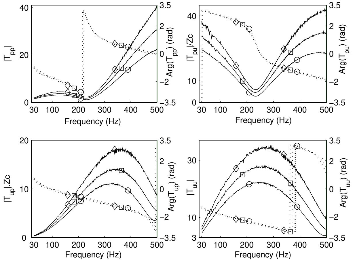
Figure 3.34: Stainless Steel Grids: amplitude (solid line) and phase (dotted line) of the T_{TAC} coefficients in the frequency domain for Q_H = 0\text{ W} (circle), Q_H = 36\text{ W} (square) and Q_H = 72\text{ W} (diamond) - Impedance Method.
