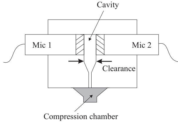
Figure B.1: Detail of the calibration device showing the two micros and the small cavity as the coupling volume submitted to uniform acoustic pressures provided by the compression chamber.
