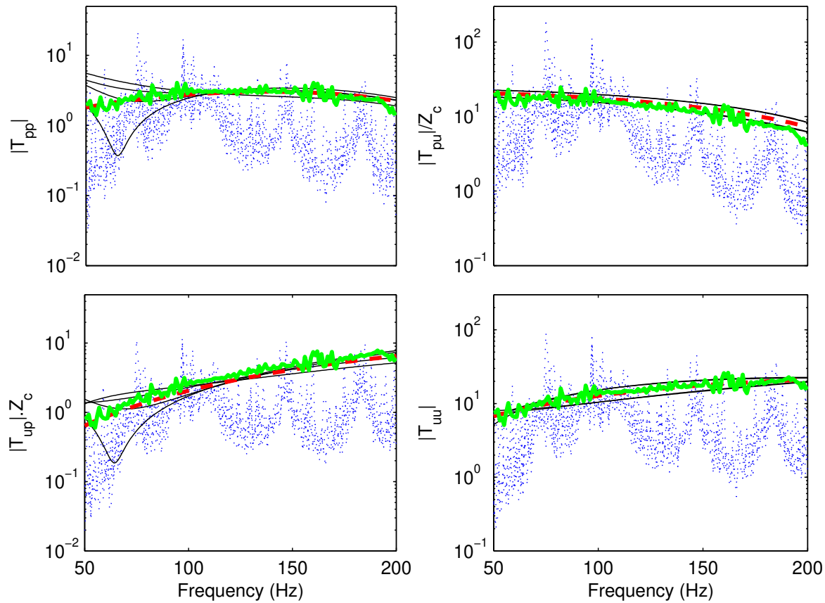
Figure 3.19: Stainless Steel Grids: amplitude of the four \mathcal{T} coefficients in the frequency domain for Q_H = 0 W in bold lines for the measurements (solid) and theory (dashed), with the respective theoretical bias (four thin solid lines per graph) and noise (five dotted lines per graph). - Two-Load Method.
