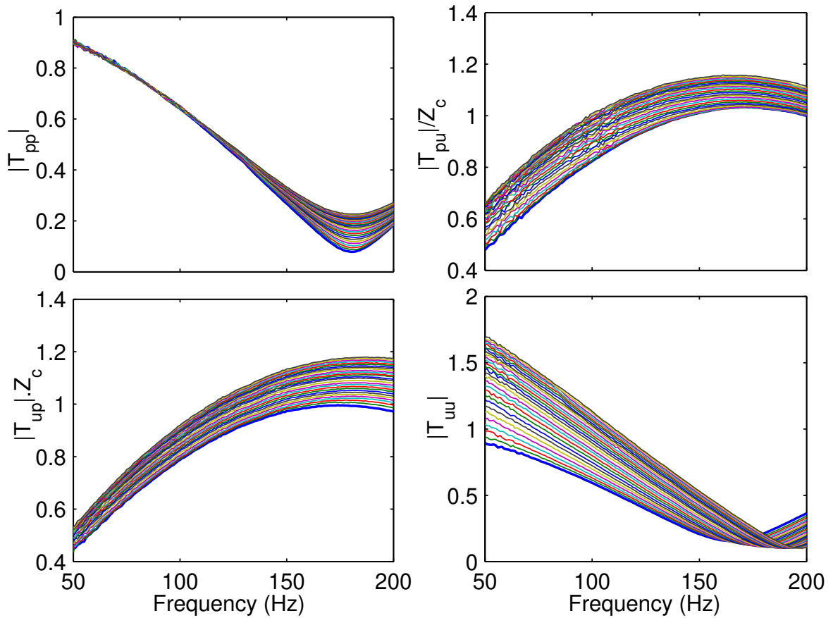
Figure D.1: Ceramic Catalyst 600 CPSI: amplitude of the four \mathcal{T} coefficients in the frequency domain for Q_H ranging from 0W to 81W , by a constant increment of 3W . The bold graph line corresponds to Q_H = 0W . - Two-Load Method.
