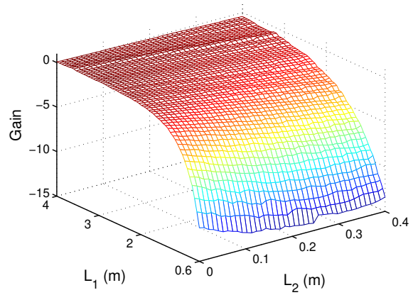
Figure 4.5: Gain for standing-wave engines at Q_H = 0 W from measured T_{TAC} of the Ceramic Catalyst by the Impedance Method.
