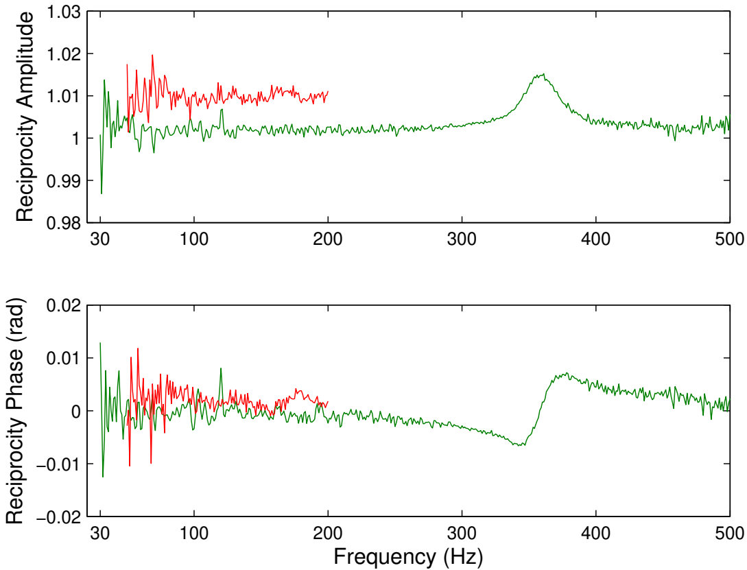
Figure 3.40: Ceramic Catalyst: amplitude and phase of the T_{TAC} reciprocity in the frequency domain for Q_H = 0 W for the Impedance Method and for the Two-Load Method (lines of narrower frequency range).
