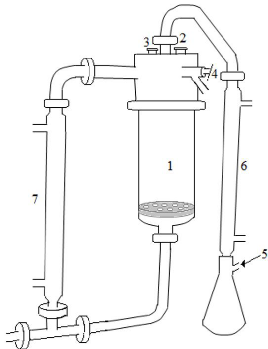
Figure 1. Osmotic Dehydration equipment: 1 – Vessel (capacity = 3L); 2 – connection for pressure meter; 3 – connection for thermostat; 4 – breaking vacuum; 5 – connection for vacuum pump; 6 – condenser; 7 – tubular heat exchanger.
