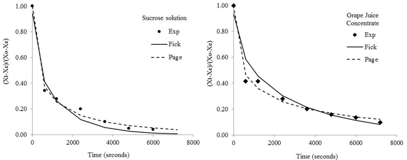
Figure 3. Moisture variation (dimensionless) over time of osmotically dehydrated melon with sucrose solution and grape juice concentrate versus time. X_o , X_t e X_e are initial moisture content (g/g, d.b.), moisture content at instant t (g/g, d.b.) and equilibrium moisture content (g/g, d.b.), respectively.
