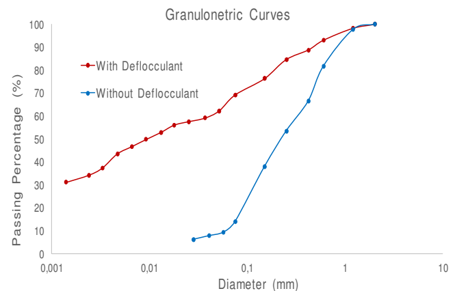
Figure 1. Grain-size distribution curves with and without deflocculant (trench 4, B horizon)
