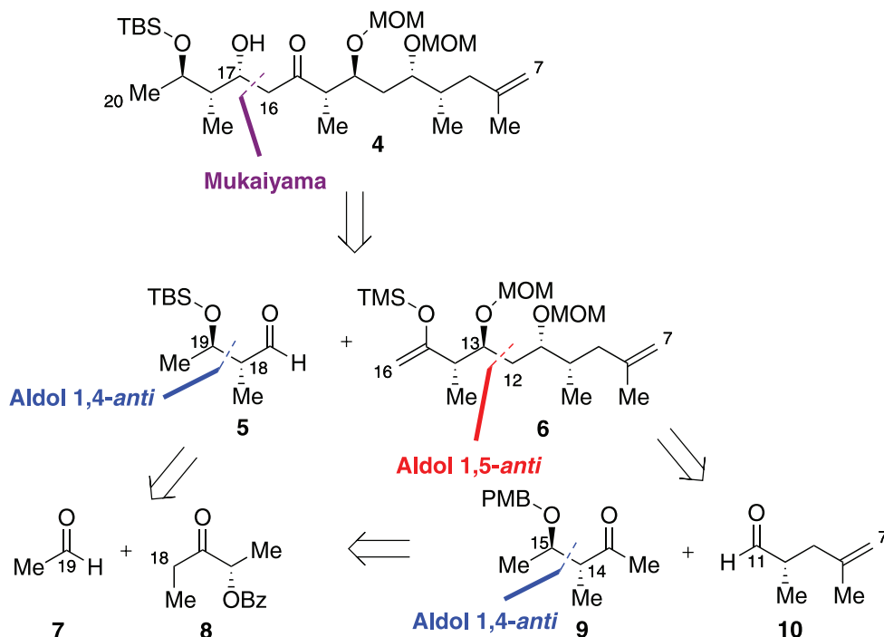
Scheme 1. Retrosynthetic analysis.
