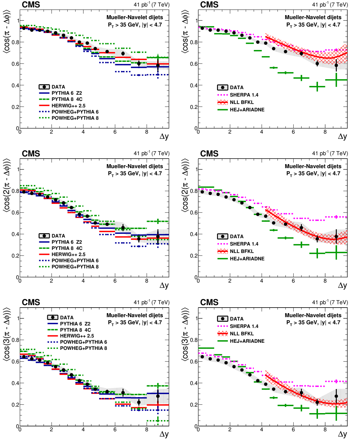
Figure 2. Left: average \langle \cos(n(\pi - \Delta\phi)) \rangle ( n = 1, 2, 3 ) as a function of \Delta y compared to LL DGLAP MC generators. In addition, the predictions of the NLO generator POWHEG interfaced with the LL DGLAP generators PYTHIA 6 and PYTHIA 8 are shown. Right: comparison of the data to the MC generator SHERPA with parton matrix elements matched to a LL DGLAP parton shower, to the LL BFKL inspired generator HEJ with hadronisation by ARIADNE, and to analytical NLL BFKL calculations at the parton level ( 4.0 < \Delta y < 9.4 ).
