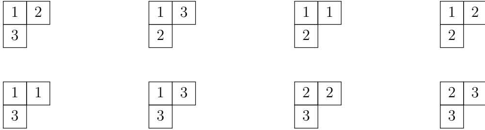
Figura 7 – (2, 1) -tabelas semistandard.
