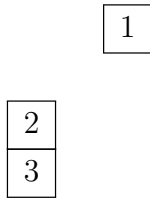
Figura 22 – T_{(3,2,1^2) \setminus (2^2)}
