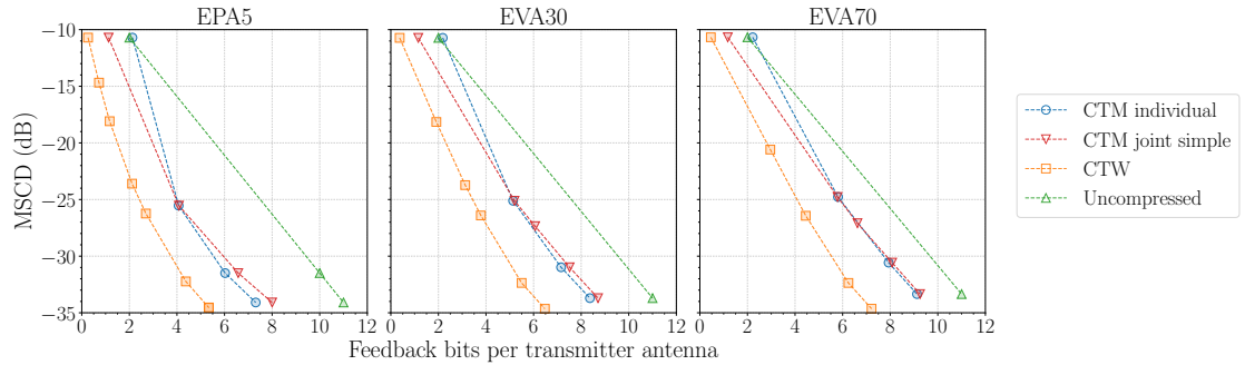
Fig. 8: MSCD distortion using \beta -law compander, for N_t = 16 , N_r = 8 .
