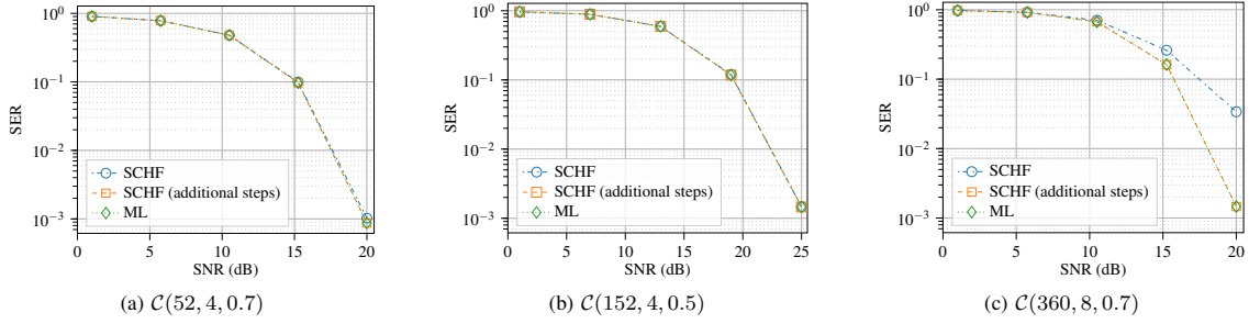
Fig. 9. Symbol error rate (SER) for decoding different SCHF C(M, n, d) with sub-optimal SCHF methods and brute-force ML decoder.
