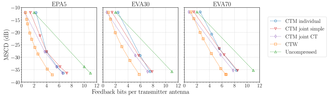
Fig. 7: MSCD distortion using \beta -law compander, for N_t = 4 , N_r = 4 .
