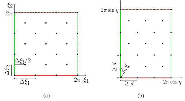
Fig. 3. Distribution of points on a torus T_\eta , seen as the preimage by \iota_\eta (a) and \Phi_c (b), where c = (\cos \eta, \sin \eta) . In this case, d = 0.9 and \eta = 2 \arcsin(d/2) , so that m = 3 and n = 6 . Moreover, \Delta\xi_1 = 2\pi/m = 2\pi/3 and \Delta\xi_2 = 2\pi/n = \pi/3 . Note the displacement of \Delta\xi_1/2 between consecutive internal circles.
