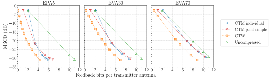
Fig. 7: MSCD distortion using \beta -law compander, for N_t = 4 , N_r = 4 .
