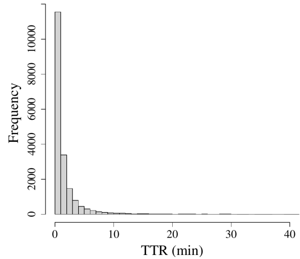
Figure A.16: Histogram of TTR data for Line A Labeller 2.
