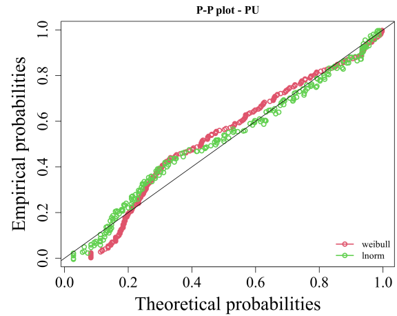
Figure D.24: P-P plot for the Pasteurization Unit TTR data - comparison between Log-normal and Weibull.
