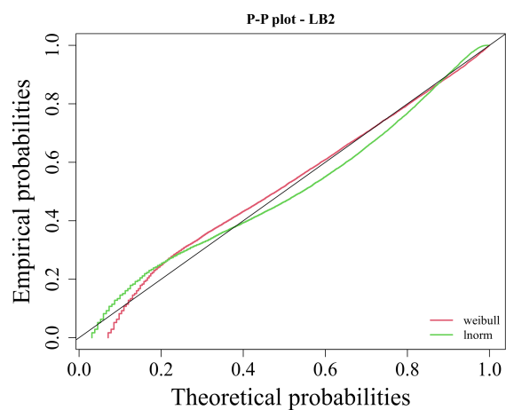
Figure D.30: P-P plot for the Labeller 2 TBF data - comparison between Log-normal and Weibull.
