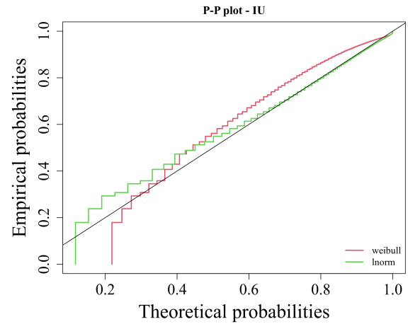
Figure D.16: P-P plot for the Inspector Unit TTR data - comparison between Log-normal and Weibull.
