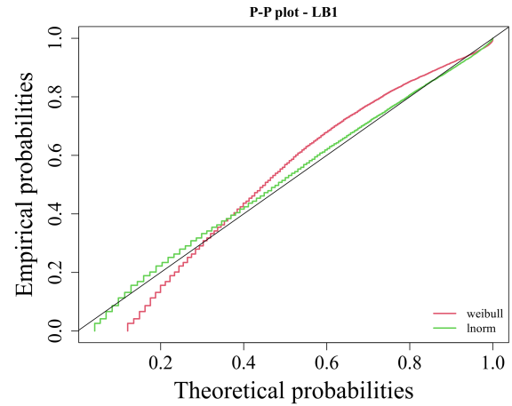
Figure D.28: P-P plot for the Labeller 1 TTR data - comparison between Log-normal and Weibull.
