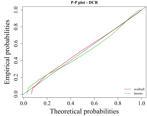
Figure D.6: P-P plot for the Decrater TBF data - comparison between Log-normal and Weibull.
