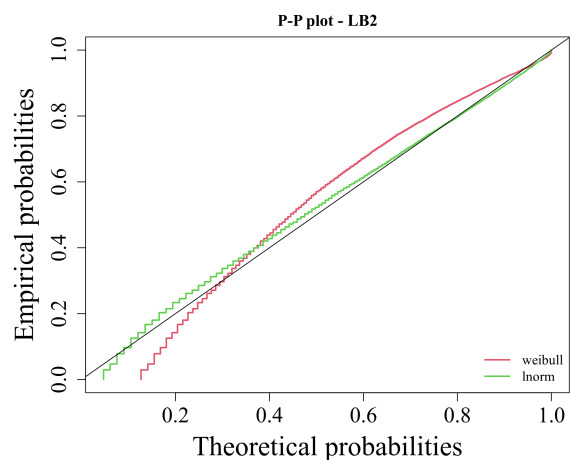
Figure D.32: P-P plot for the Labeller 2 TTR data - comparison between Log-normal and Weibull.
