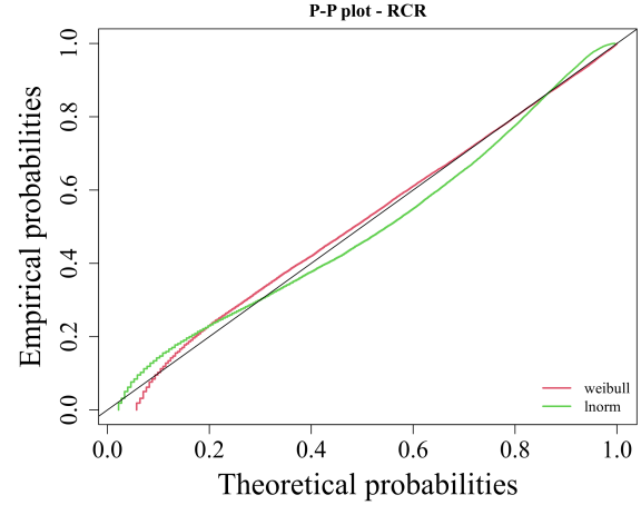
Figure D.34: P-P plot for the Recrater TBF data - comparison between Log-normal and Weibull.
