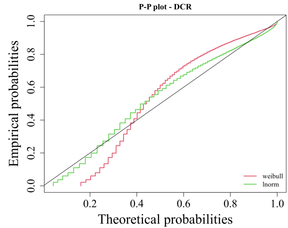
Figure D.8: P-P plot for the Decrater TTR data - comparison between Log-normal and Weibull.
