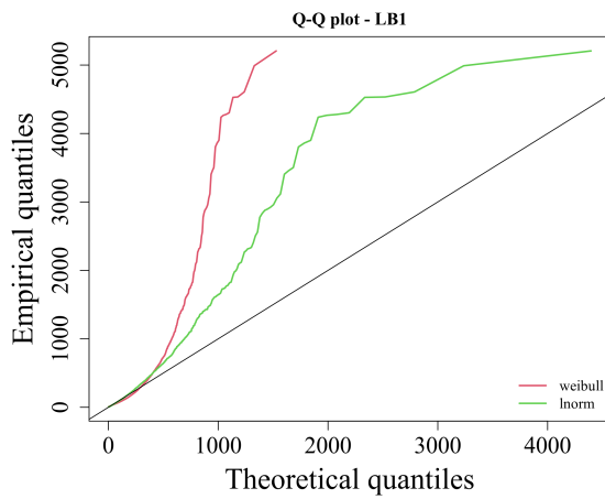
Figure D.27: Q-Q plot for the Labeller 1 TTR data - comparison between Log-normal and Weibull.
