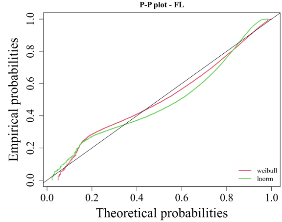
Figure D.18: P-P plot for the Filler TBF data - comparison between Log-normal and Weibull.
