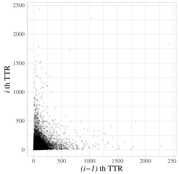
Figure C.40: Line A Palletizer serial correlation for TTR data.
