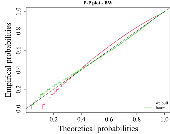
Figure D.10: P-P plot for the Bottle Washer TBF data - comparison between Log-normal and Weibull.
