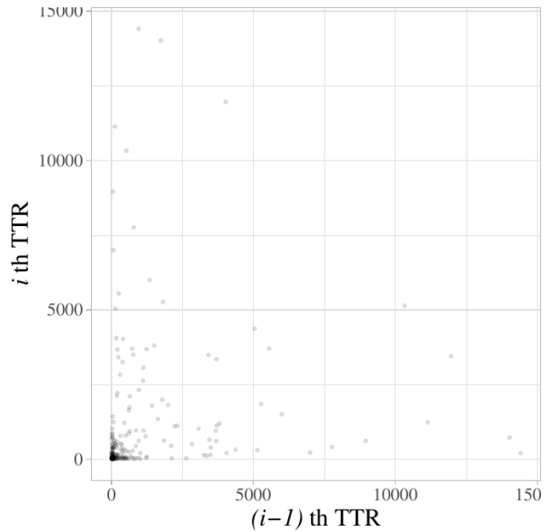
Figure C.24: Line A Pasteurization Unit serial correlation for TTR data.
