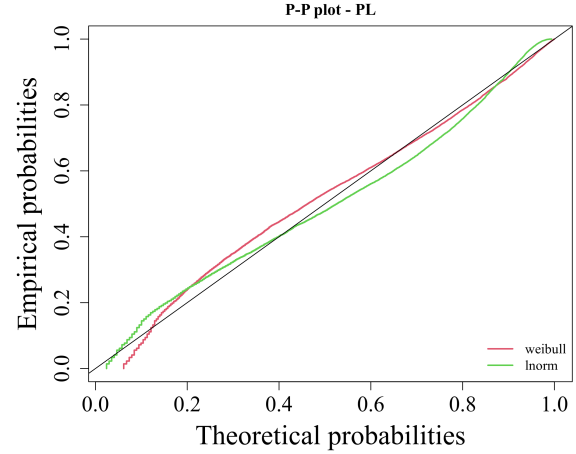
Figure D.38: P-P plot for the Palletizer TBF data - comparison between Log-normal and Weibull.
