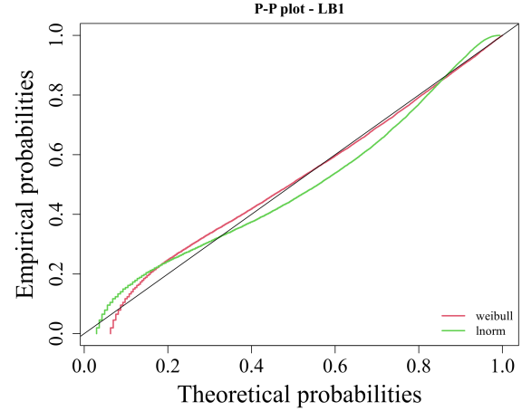
Figure D.26: P-P plot for the Labeller 1 TBF data - comparison between Log-normal and Weibull.
