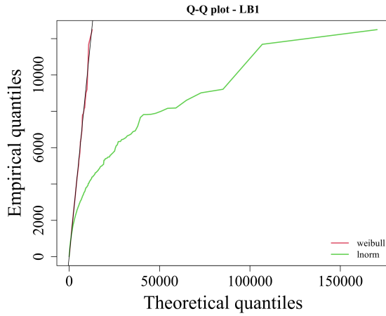
Figure D.25: Q-Q plot for the Labeller 1 TBF data - comparison between Log-normal and Weibull.
