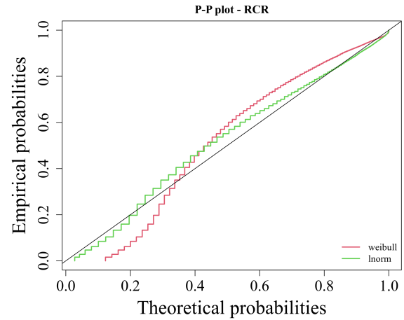
Figure D.36: P-P plot for the Recrater TTR data - comparison between Log-normal and Weibull.
