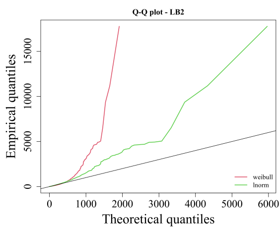
Figure D.31: Q-Q plot for the Labeller 2 TTR data - comparison between Log-normal and Weibull.
