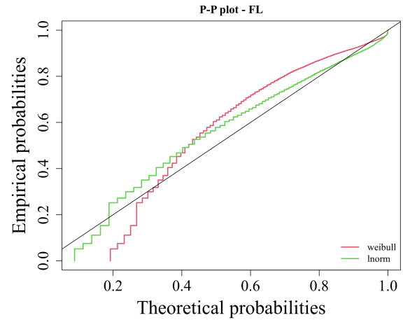
Figure D.20: P-P plot for the Filler TTR data - comparison between Log-normal and Weibull.
