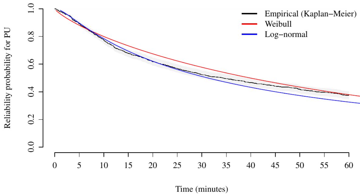
Figure 6.41: Pasteurization unit reliability plot.
