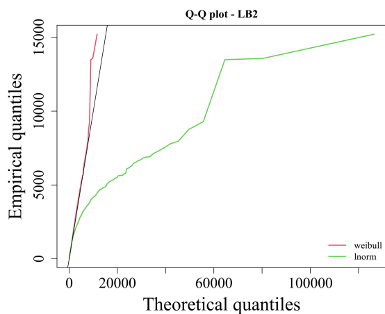
Figure D.29: Q-Q plot for the Labeller 2 TBF data - comparison between Log-normal and Weibull.
