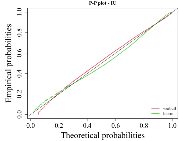
Figure D.14: P-P plot for the Inspector Unit TBF data - comparison between Log-normal and Weibull.
