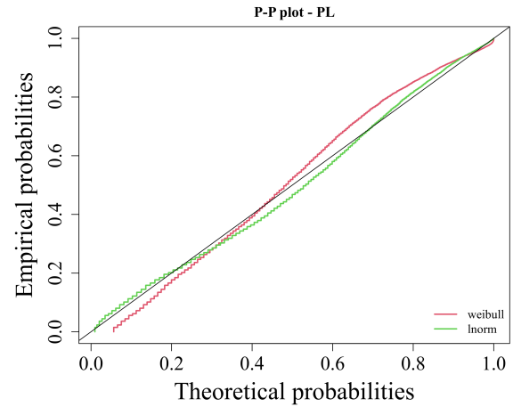
Figure D.40: P-P plot for the Palletizer TTR data - comparison between Log-normal and Weibull.
