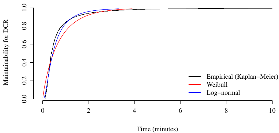
Figure G.2: Decrater maintainability plot.
