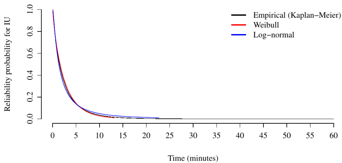
Figure F.4: Inspector Unit reliability plot.
