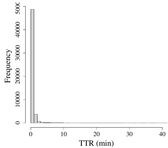
Figure A.8: Histogram of TTR data for Line A Inspector Unit.
