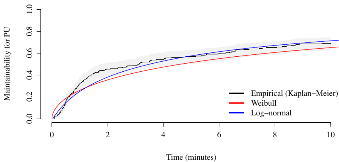
Figure G.6: Pasteurization Unit maintainability plot.
