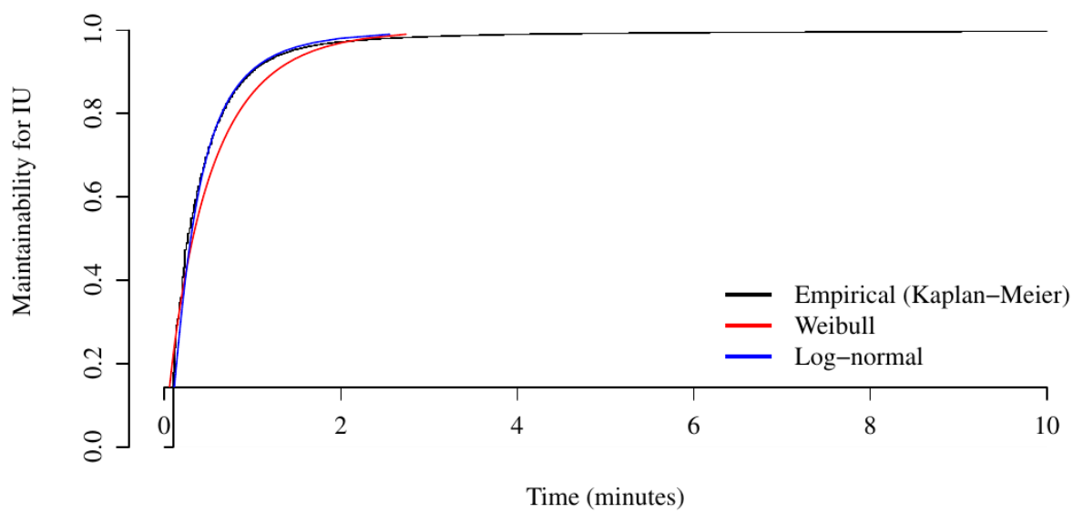
Figure G.4: Inspector Unit maintainability plot.
