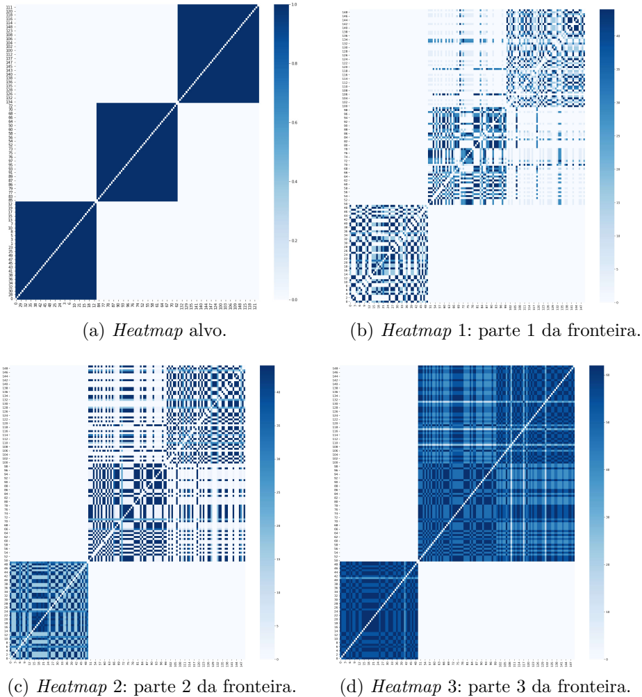
Figura 38 – Heatmaps Iris .
